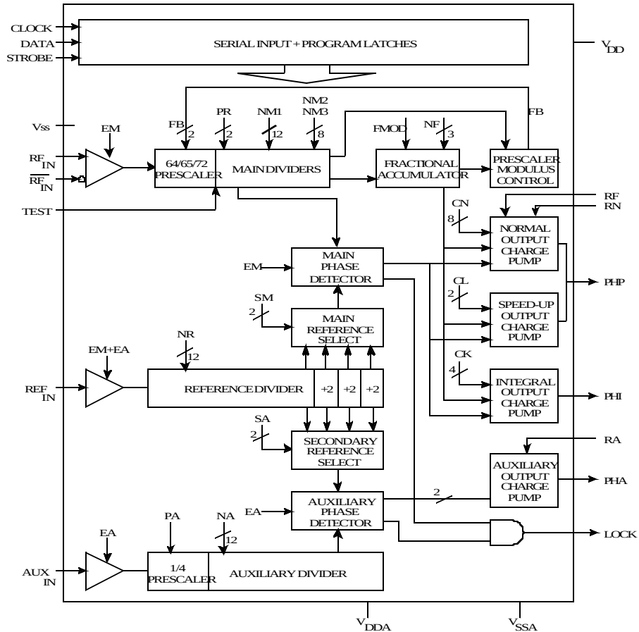
Figure 4-1 U811 Synthesizer Block Diagram
