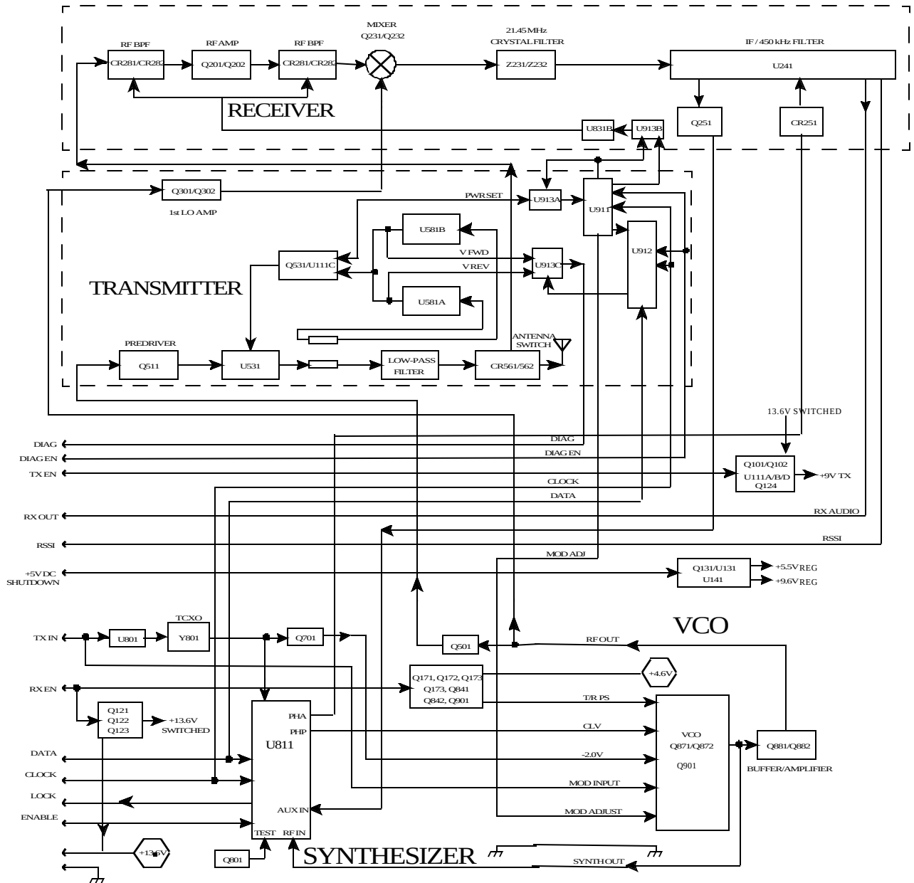
Figure 4-2 Transceiver Block Diagram
