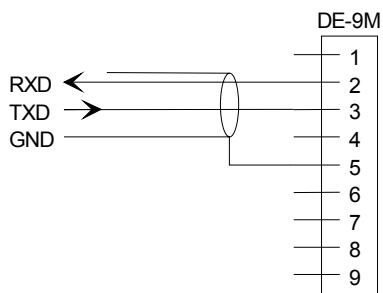
Figure 2-3 3-Wire Interface
