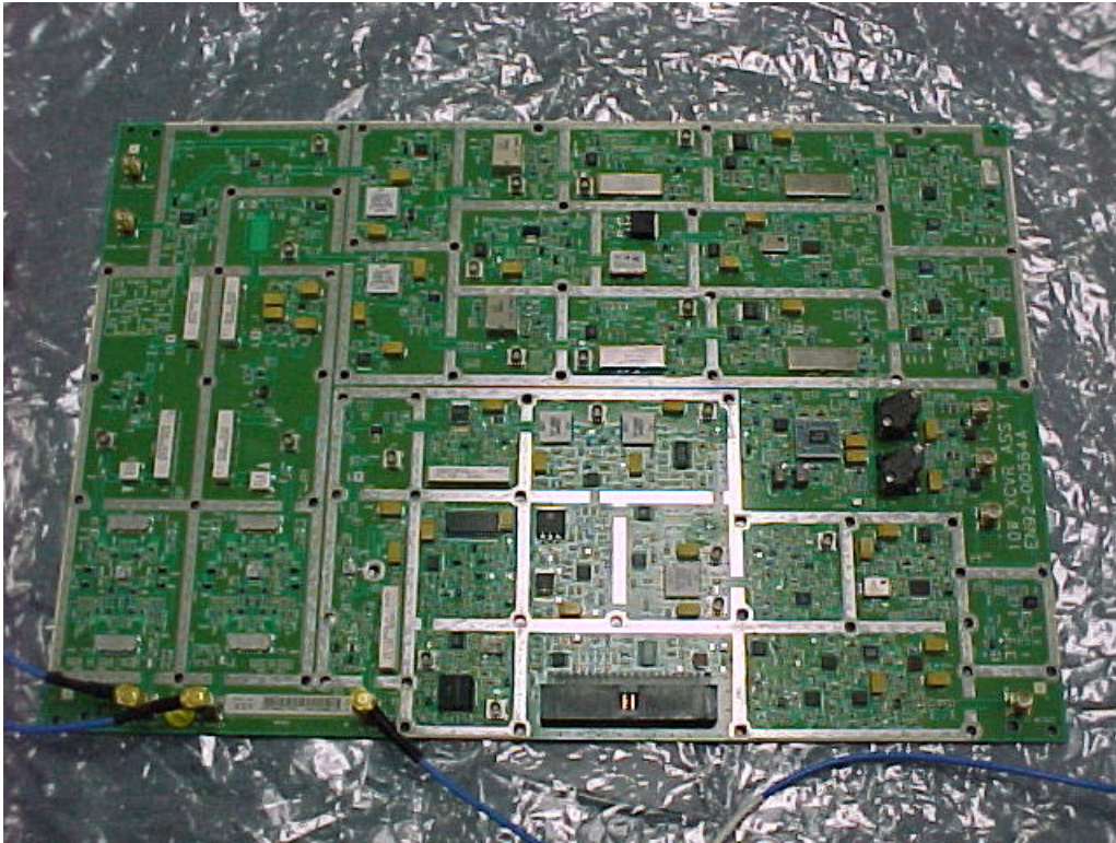
G19: PA (POWER AMPLIFIER) COVER (TOP VIEW)
