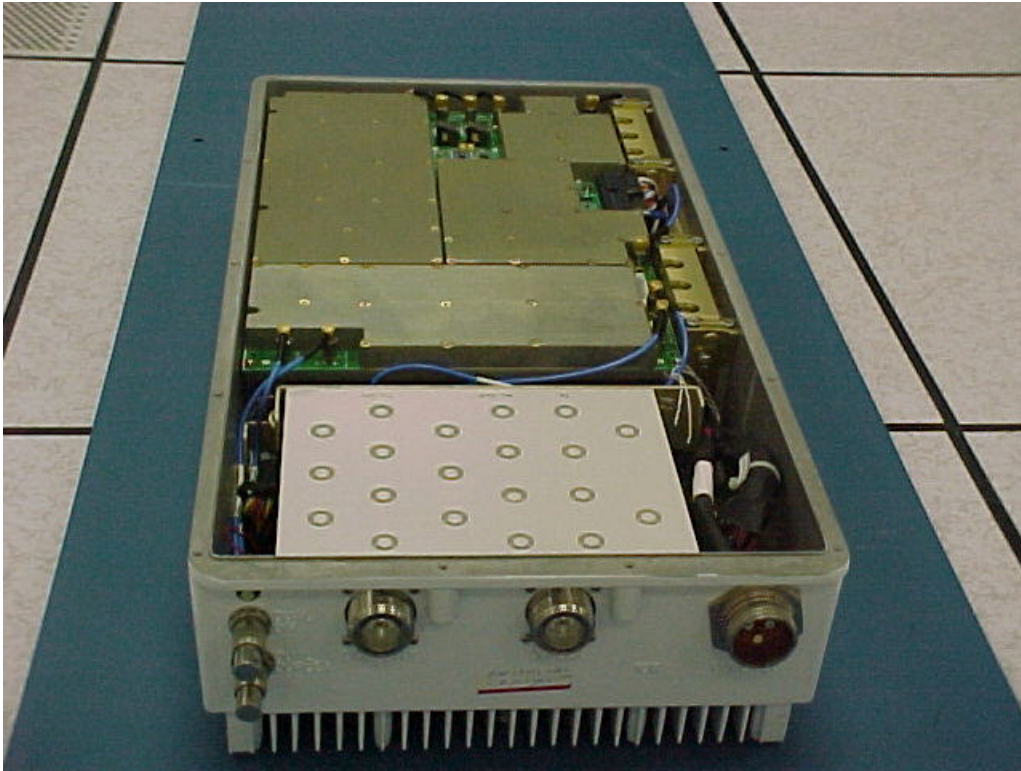
G3: UNIT ASSEMBLED (BOTTOM VIEW)
