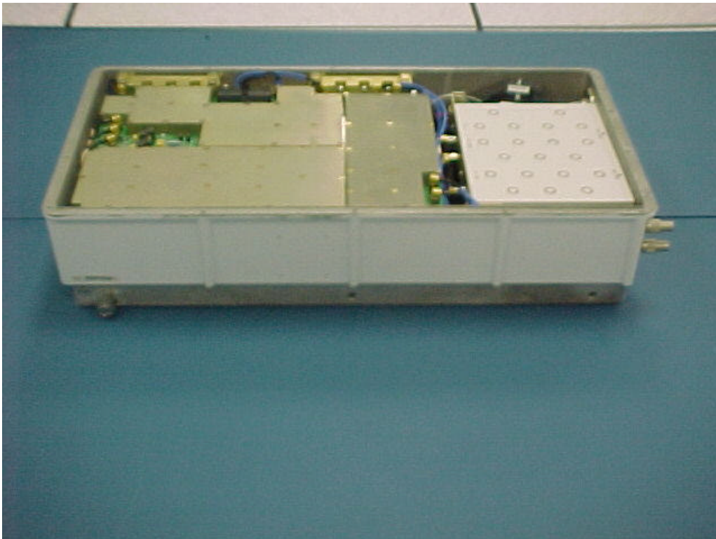
G6: UNIT ASSEMBLED (SIDE VIEW)
