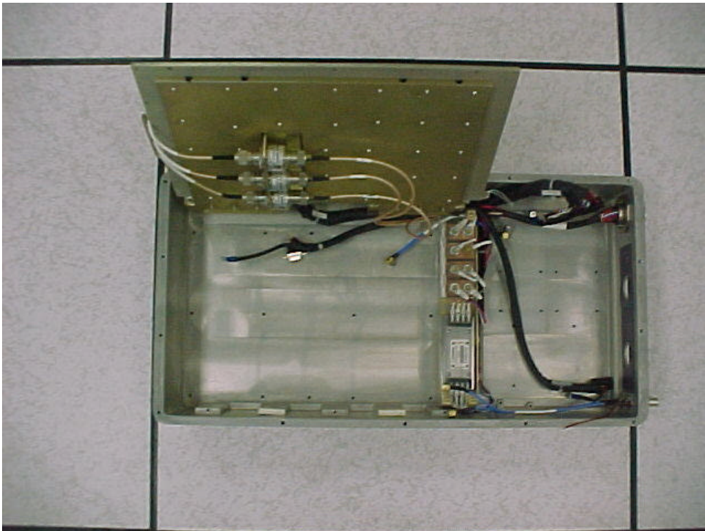
G28: HOUSING INSIDE WITH CARDS REMOVED (TOP VIEW)
