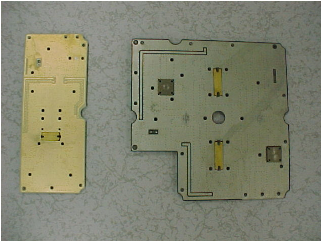
G22: POWER AMPLIFIER AND DRIVER STAGE PCB (BACK VIEW)
