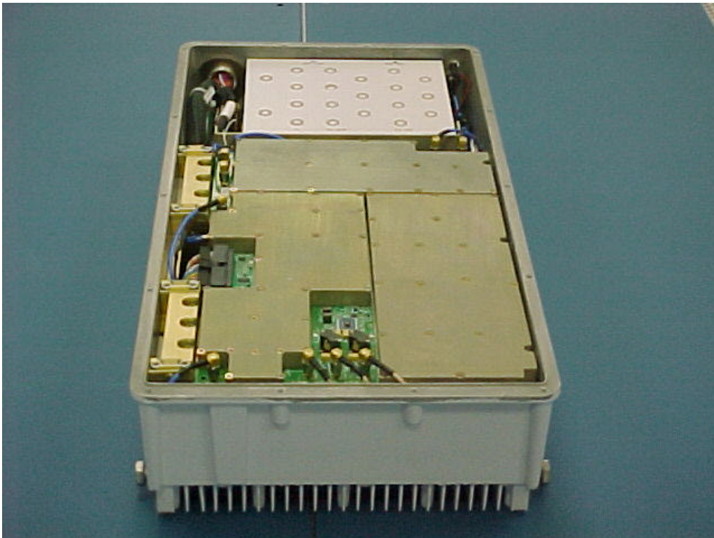
G4: UNIT ASSEMBLED (TOP VIEW)
