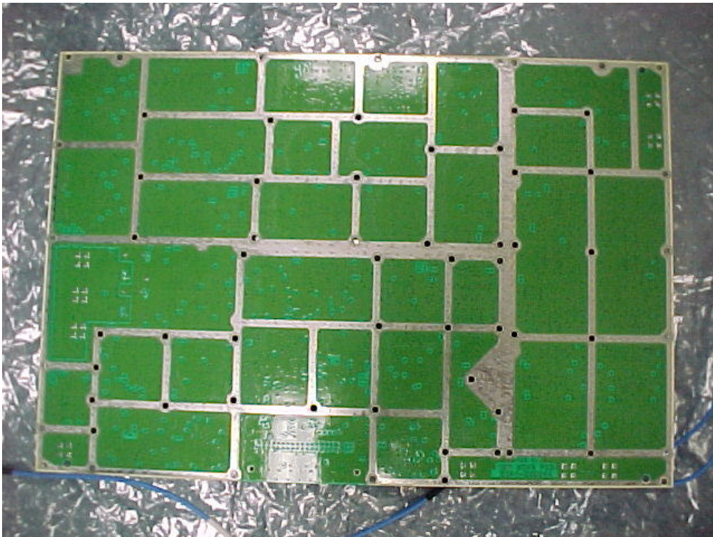
G20: TRANSCEIVER BOARD (TOP VIEW)
