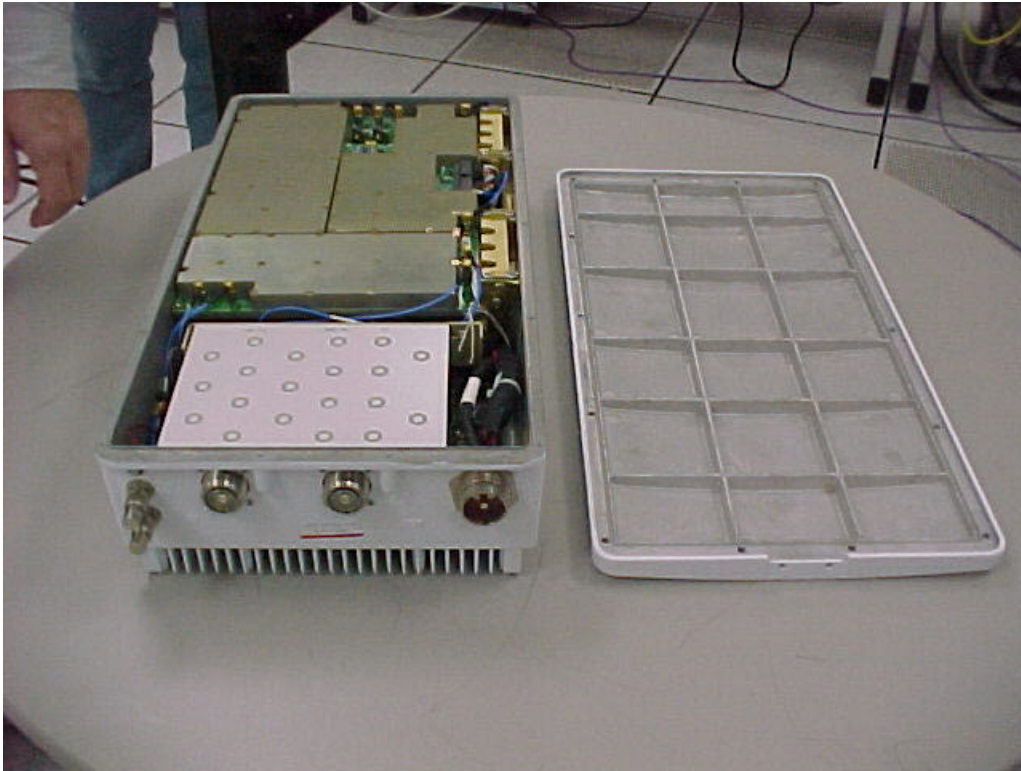
G1: UNIT ASSEMBLED (INSIDE VIEW)
