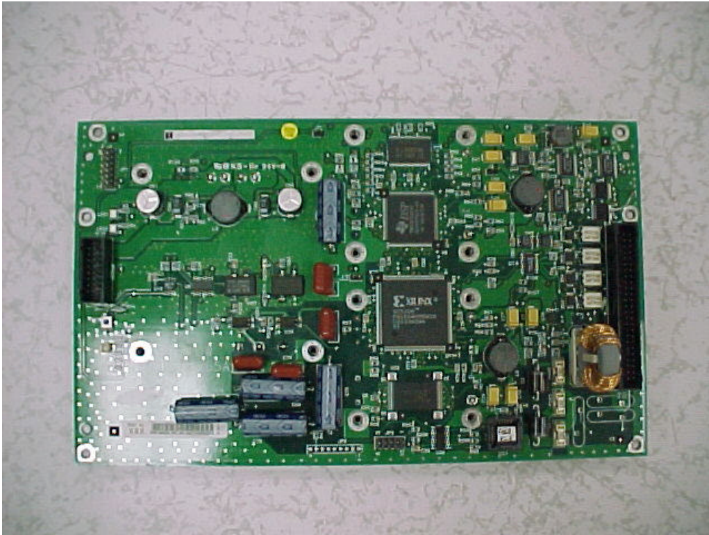
G25: PRC CARD (FRONT VIEW)
