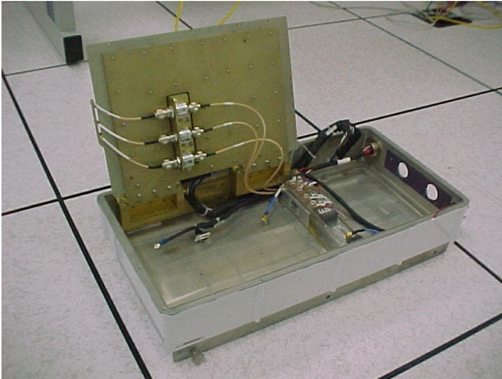
G27: INSIDE HOUSING WITH CARDS REMOVED (SIDE VIEW)
