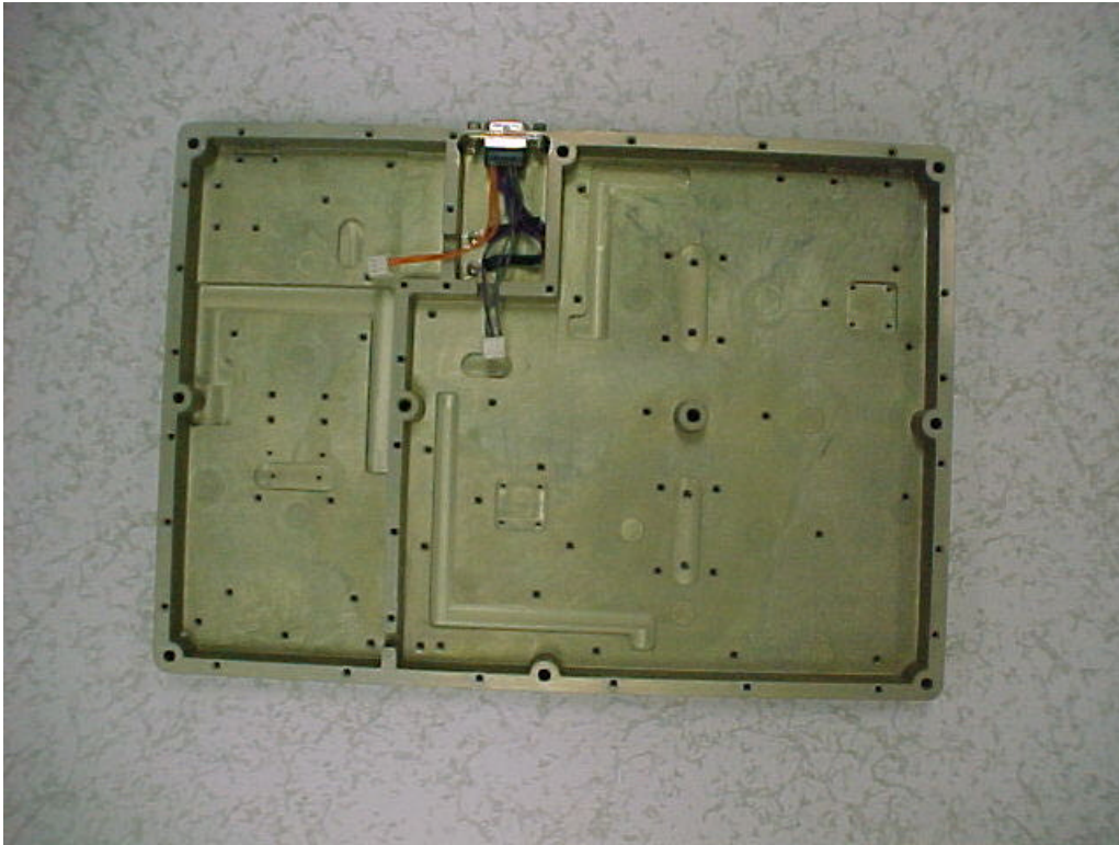
G23: POWER AMPLIFIER MODULE HOUSING (TOP/FRONT VIEW)
