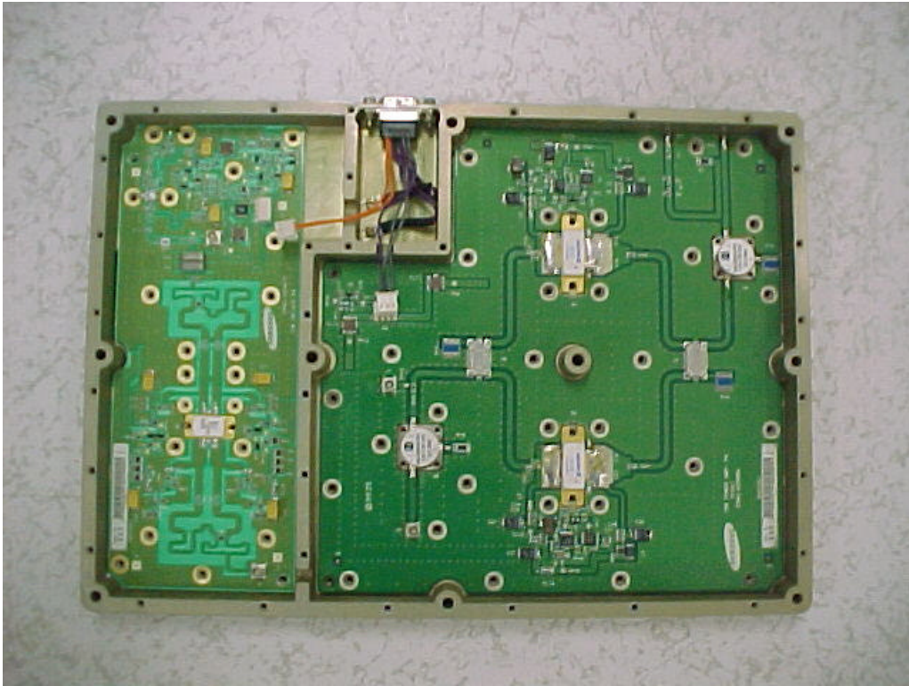
G21: POWER AMPLIFIER MODULE (TOP VIEW)
