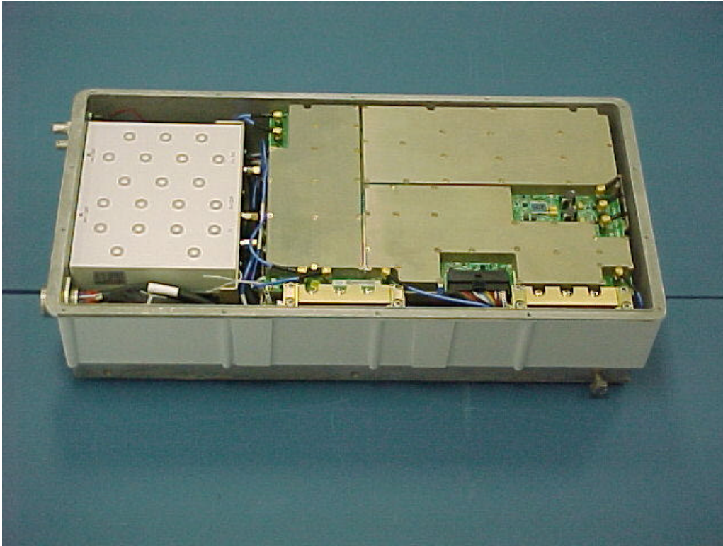
G5: UNIT ASSEMBLED (SIDE VIEW)
