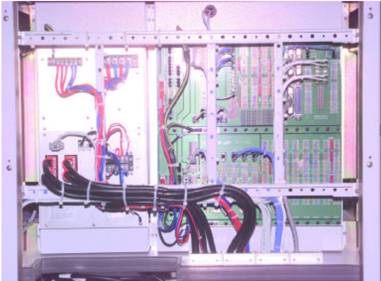
G15 : SCBS-319M-B-OPEN-UPPER
