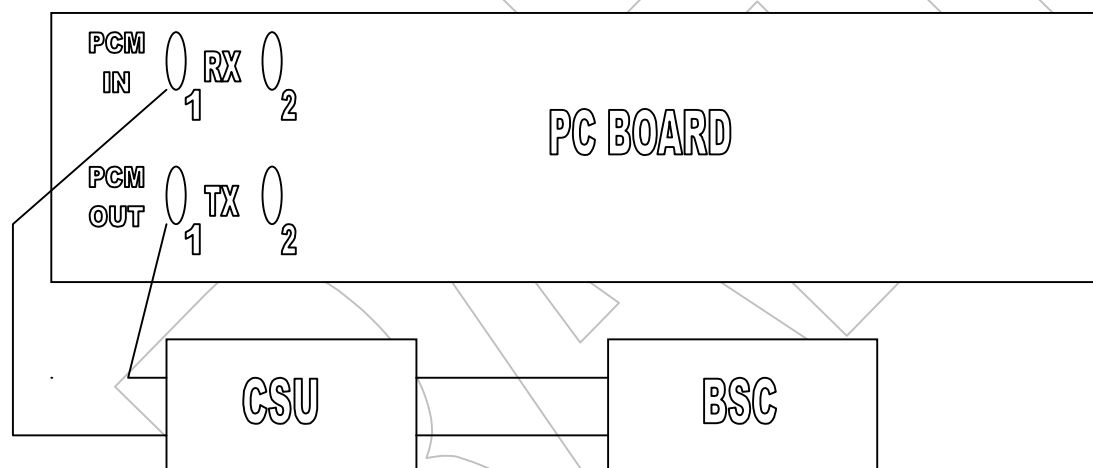
Figure 3.3 T1 Connection Backplane
