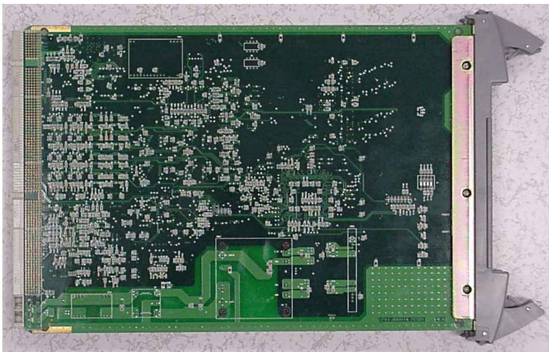
Exhibit 2 - BCAA module, trace side
