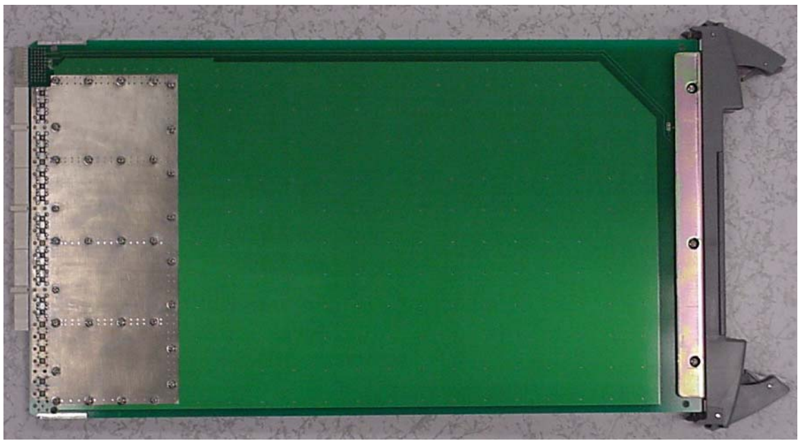
Exhibit 40 - TXCA module, trace side
