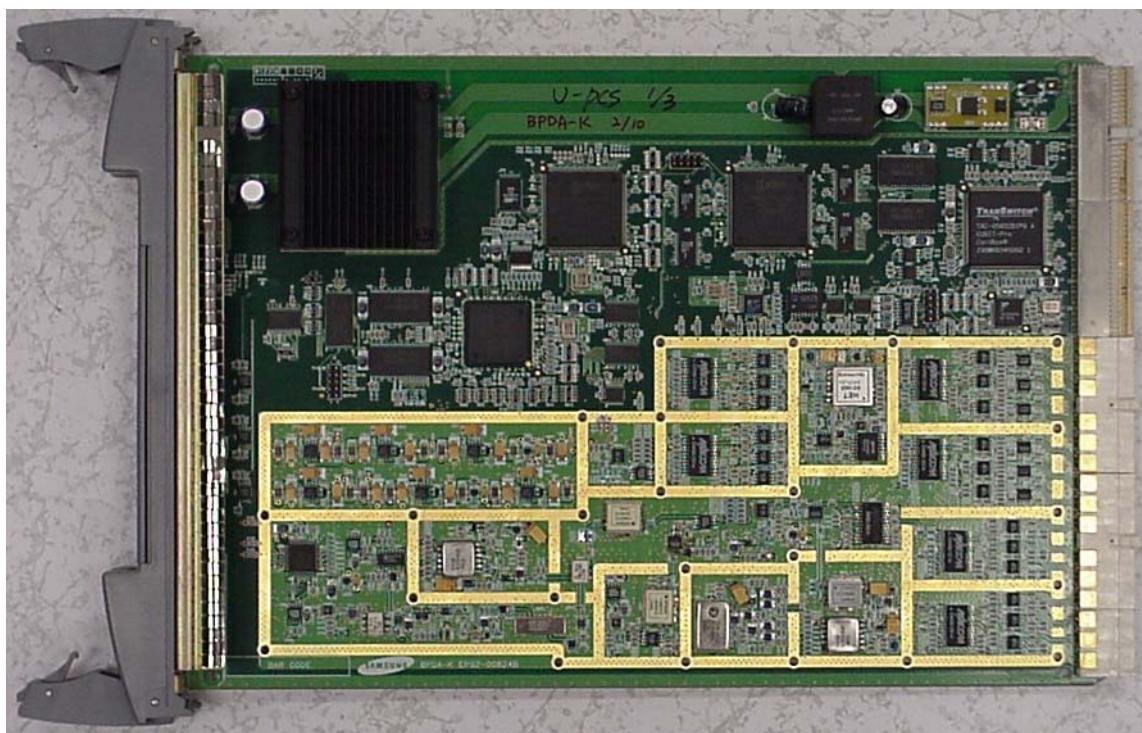
Exhibit 8 - BPDA module, component side, without cover
