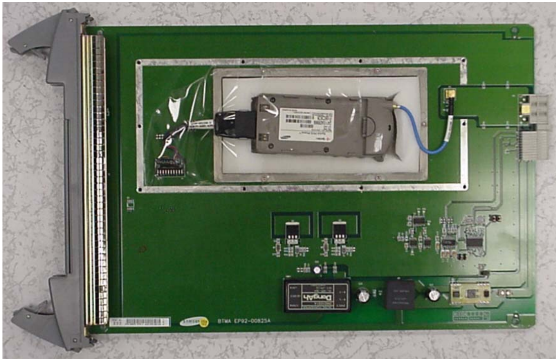
Exhibit 13 - BTMA module, component side, without cover
