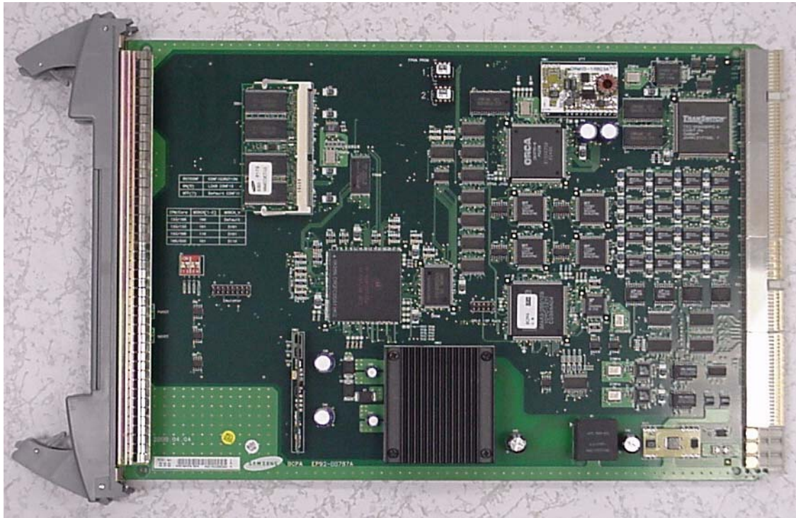
Exhibit 3 - BCPA module, component side
