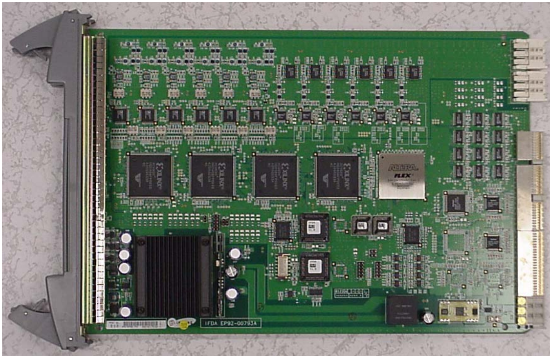
Exhibit 26 - IFDA module, component side
