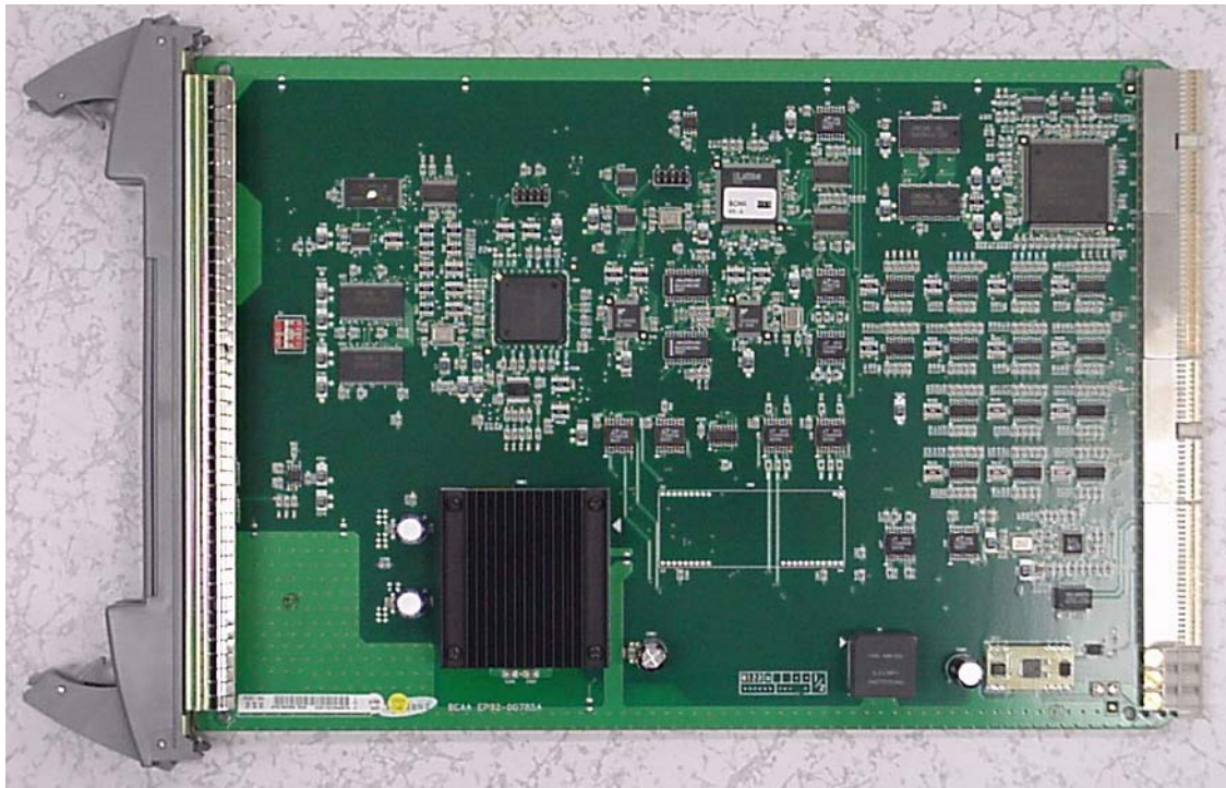
Exhibit 1 - BCAA module, component side
