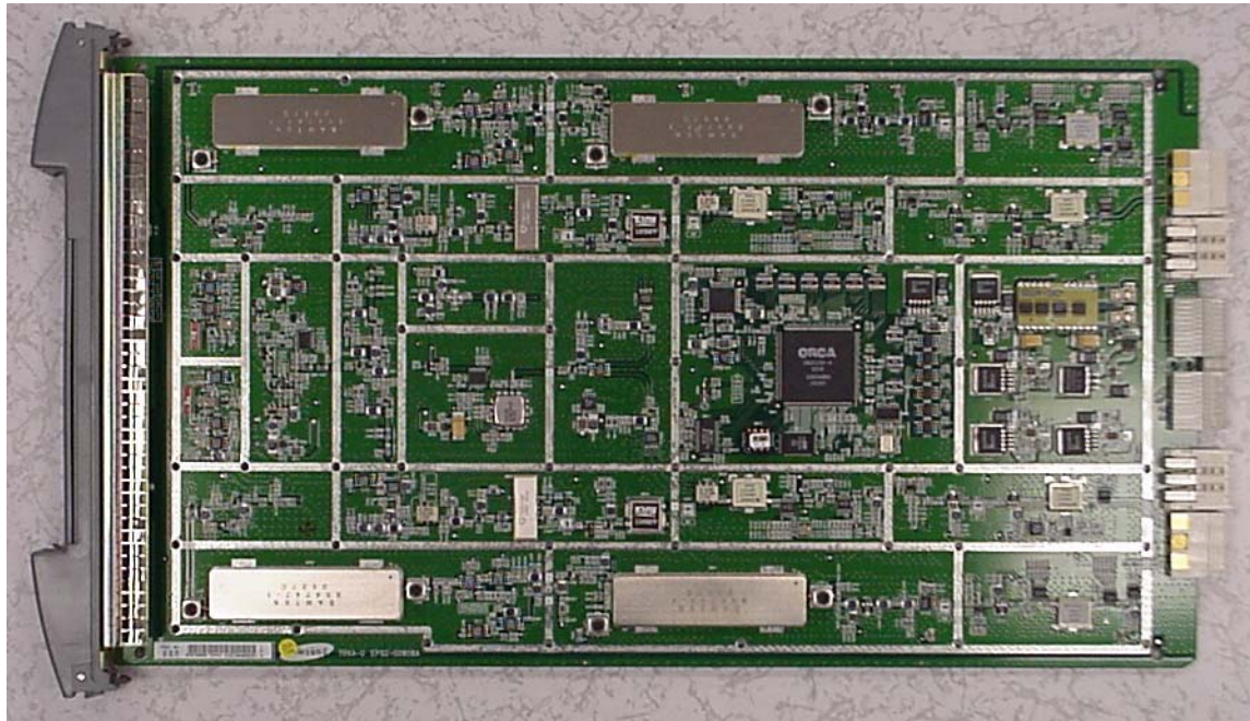
Exhibit 36 - TRXA module, component side, without cover
