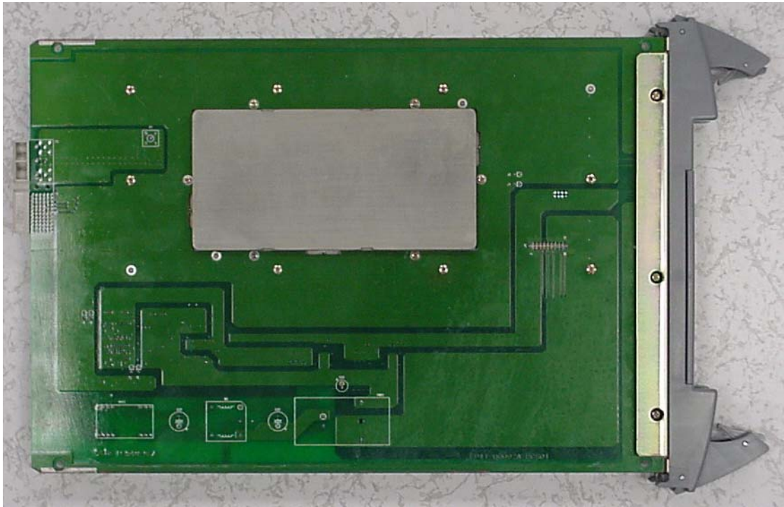
Exhibit 14 - BTMA module, trace side
