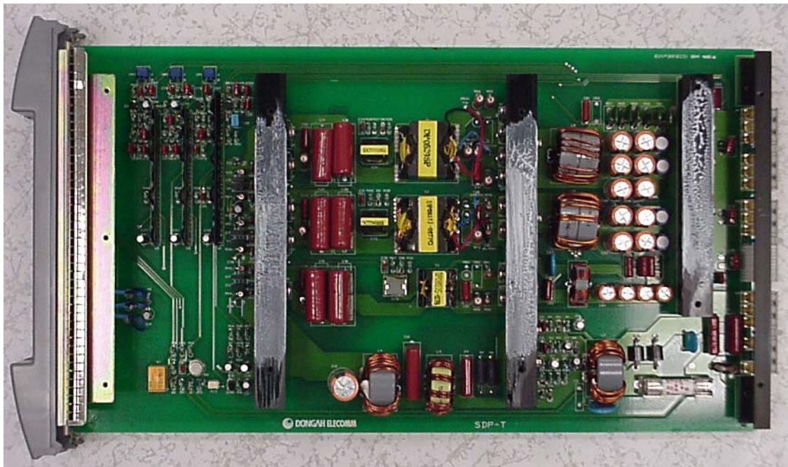
Exhibit 32 - SDP-T module, component side, without heatsink
