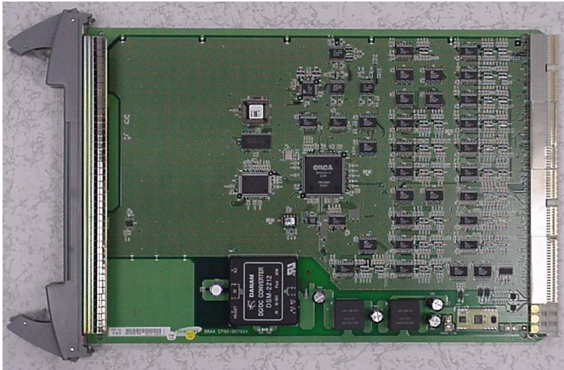
Exhibit 10 - BRAA module, component side
