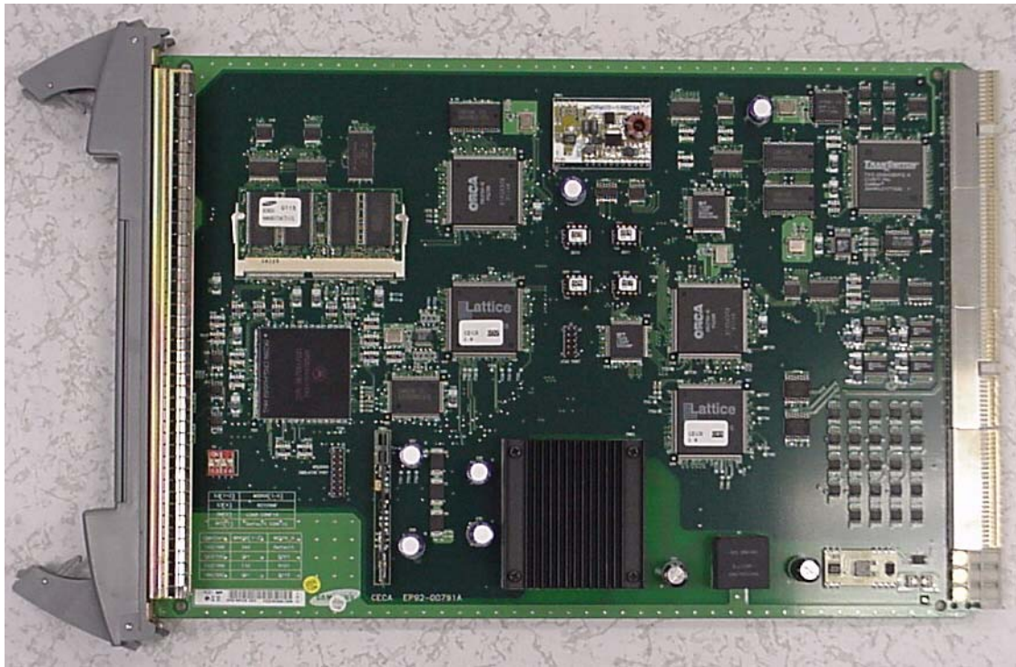
Exhibit 15 - CECA module, component side
