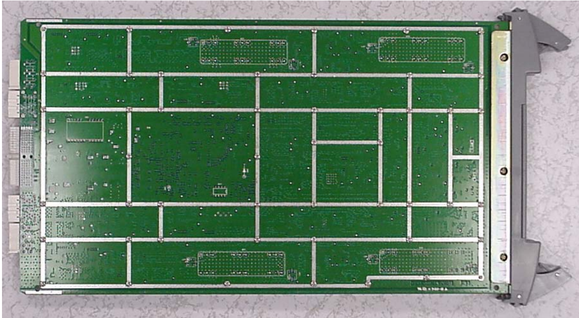
Exhibit 37 - TRXA module, trace side
