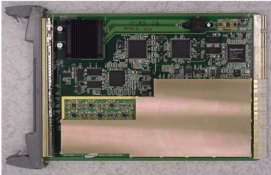
Exhibit 7 - BPDA module, component side, with cover
