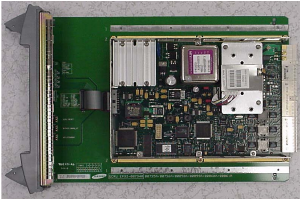
Exhibit 24 - GCRU module, component side, without cover
