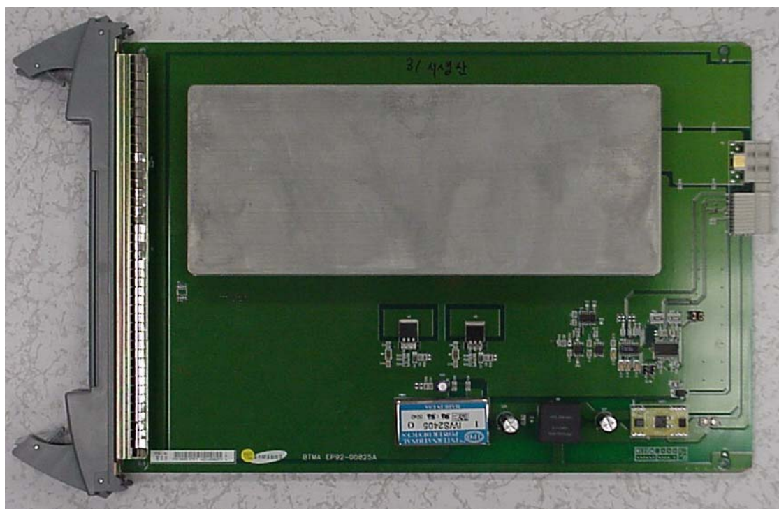
Exhibit 12 - BTMA module, component side, with cover
