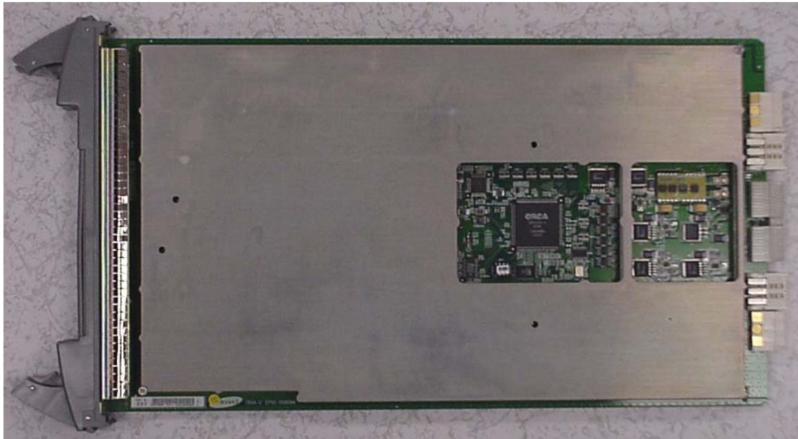
Exhibit 35 - TRXA module, component side, with cover
