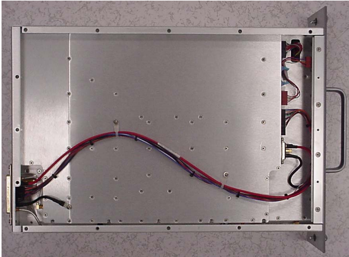
Exhibit 30 - PAU module, without cover
