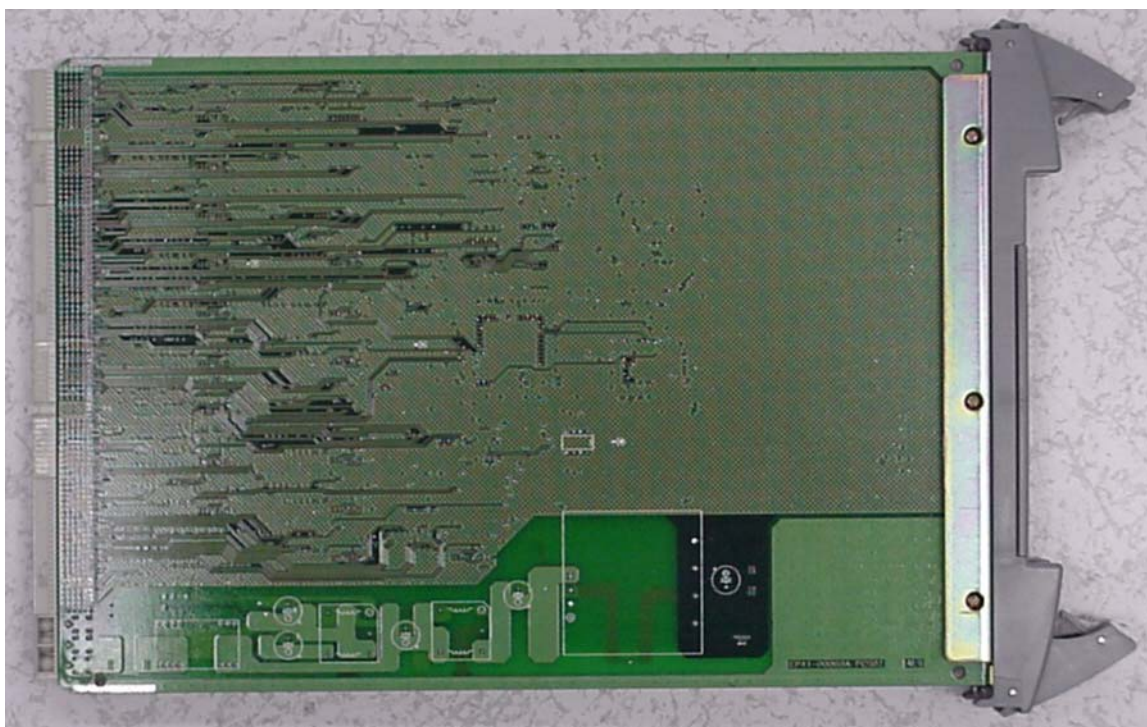
Exhibit 11 - BRAA module, trace side
