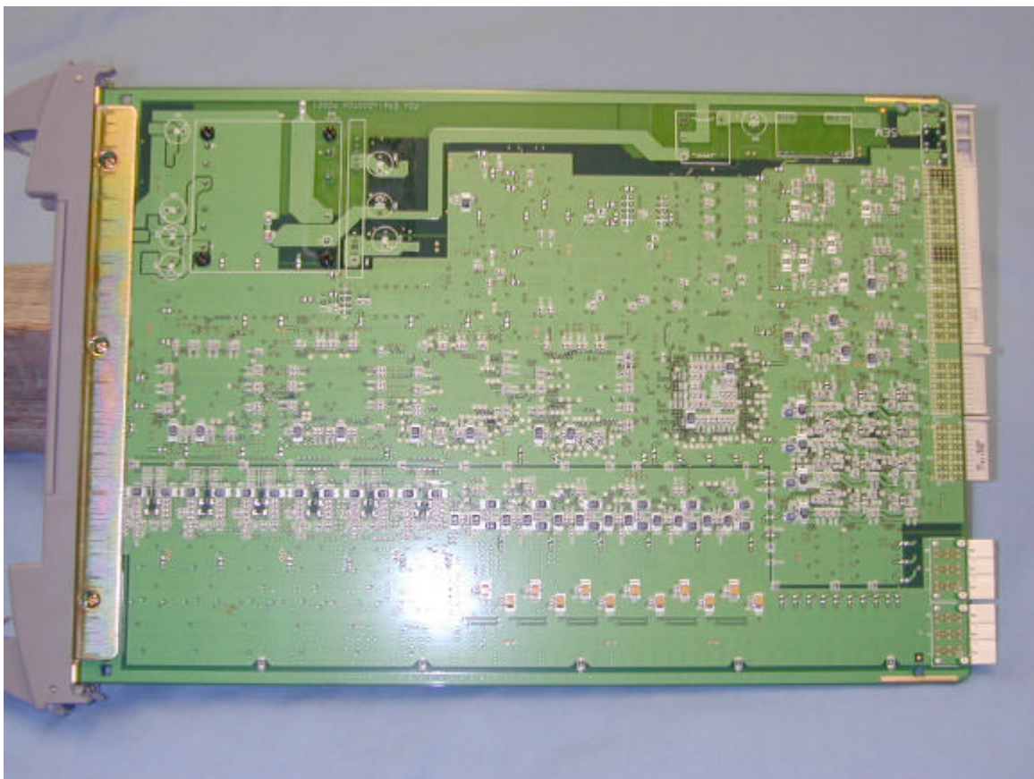
Photo 7 - IFDA Card, trace side
