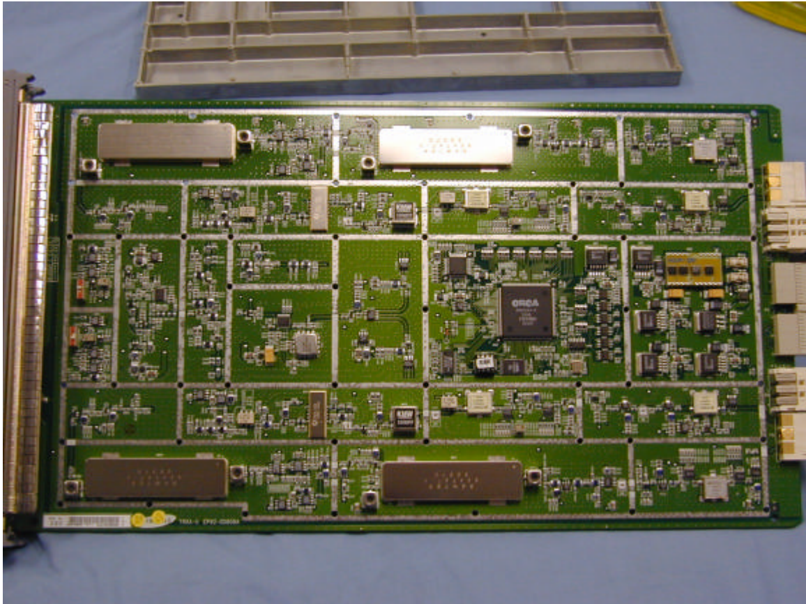
Photo 2 - Transceiver Card, without shield
