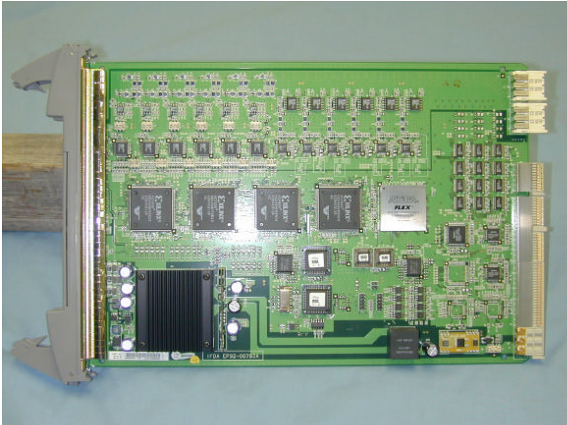
Photo 6 - IFDA Card, component side
