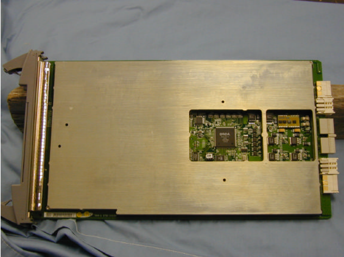
Photo 1 - Transceiver Card with shield
