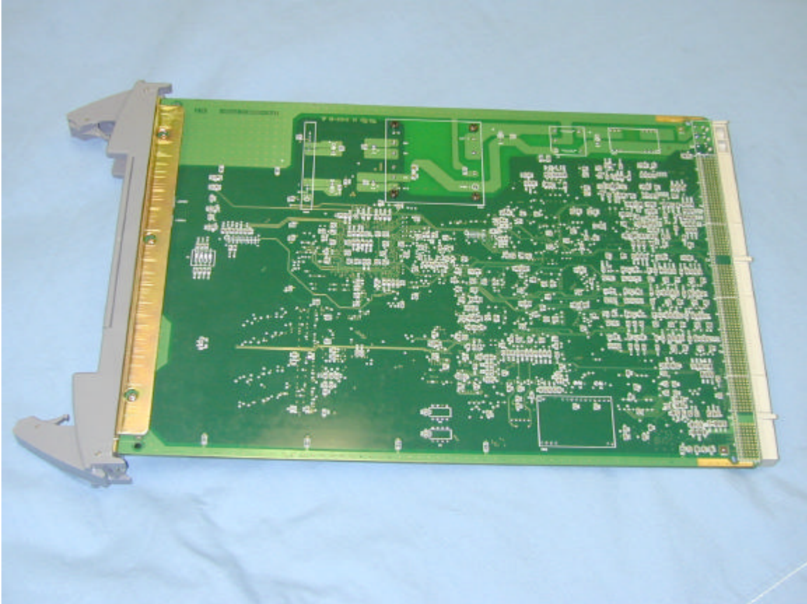
Photo 5 - BCPA Card, trace side
