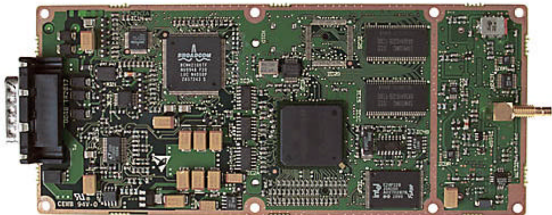
PWB, Opposite Side
