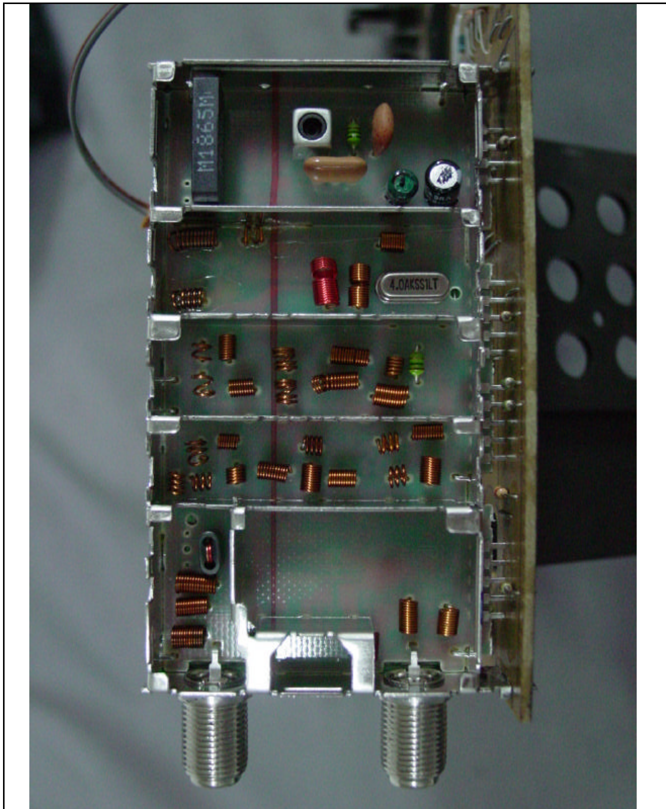
[ Top View of the TV Tuner Board ]
