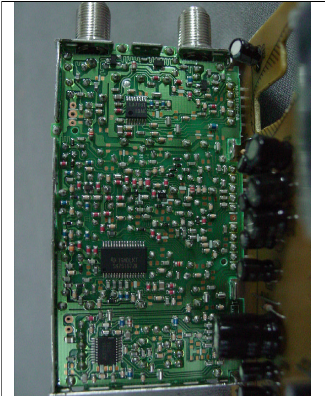
[ Bottom View of the TV Tuner Board ]
