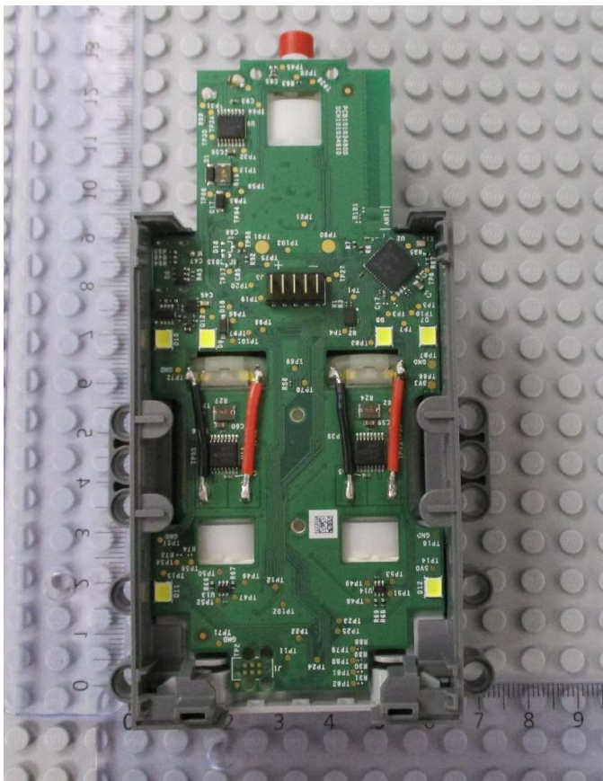
Photo of the PCBA.
