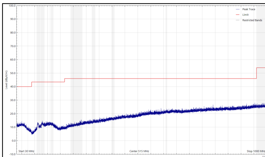
Figure 50 - CH39_LE1M_X Plane, 2480 MHz, 30 MHz to 1 GHz, Horizontal (Peak)
