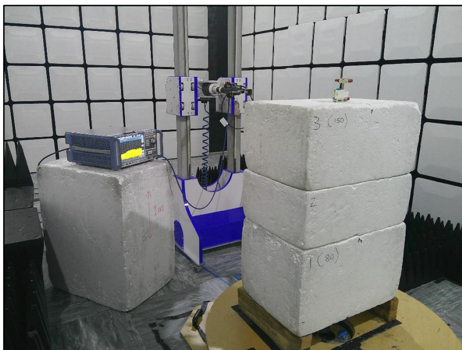
Figure 8 – Radiated Emissions - 18 GHz to 25 GHz (Y Plane)
