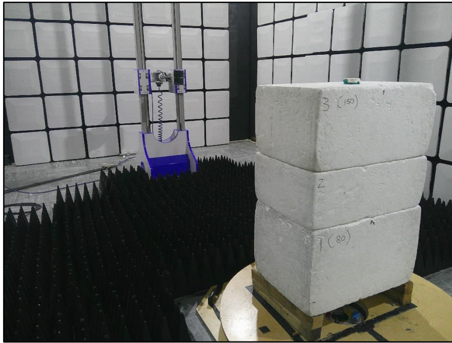
Figure 3 – Radiated Emissions - 1 GHz to 8 GHz (X Plane)
