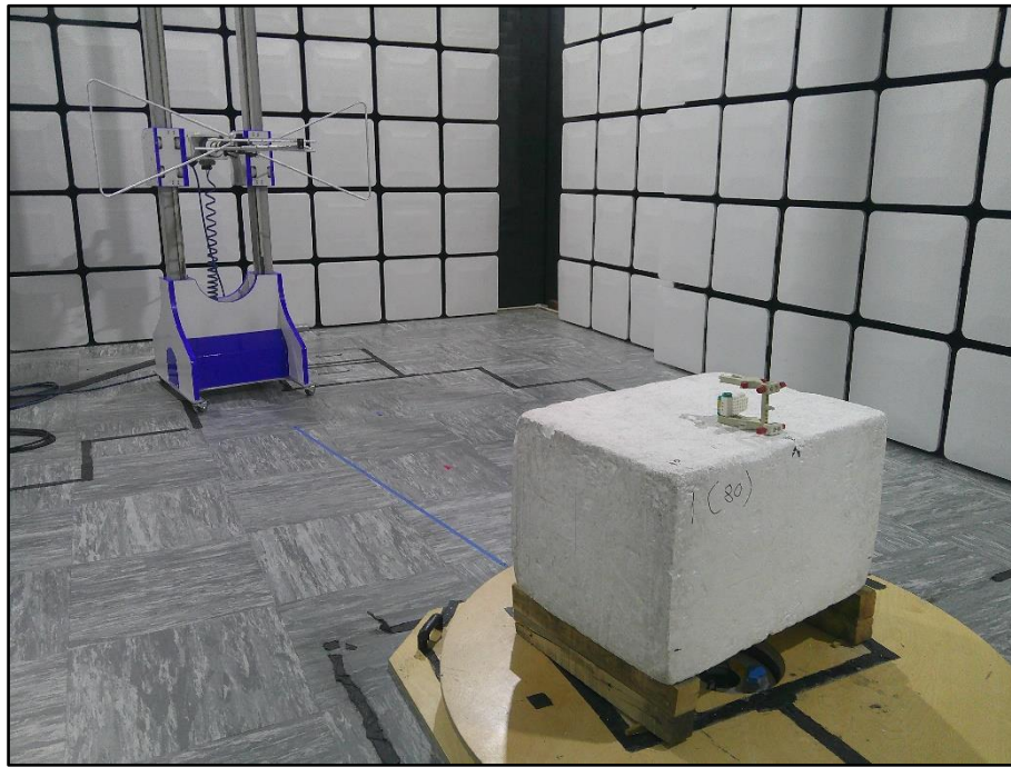
Figure 2 – Radiated Emissions - 30 MHz to 1 GHz (Y Plane)
