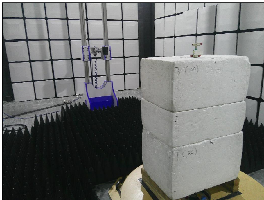
Figure 4 – Radiated Emissions - 1 GHz to 8 GHz (Y Plane)
