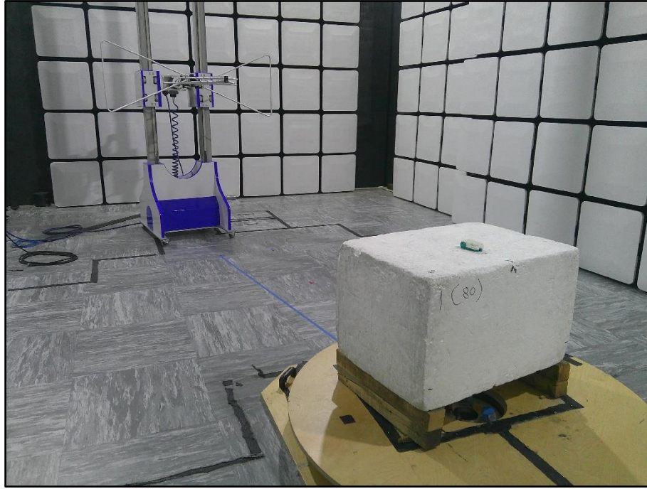
Figure 1 – Radiated Emissions - 30 MHz to 1 GHz (X Plane)
