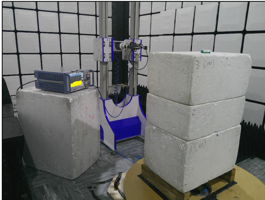
Figure 7 – Radiated Emissions - 18 GHz to 25 GHz (X Plane)
