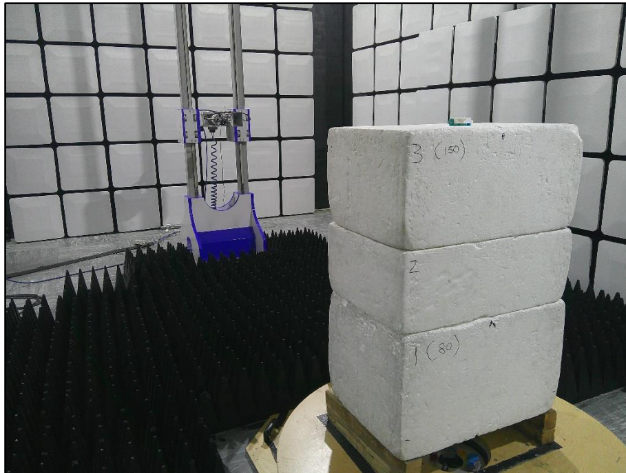
Figure 5 – Radiated Emissions - 8 GHz to 18 GHz (X Plane)
