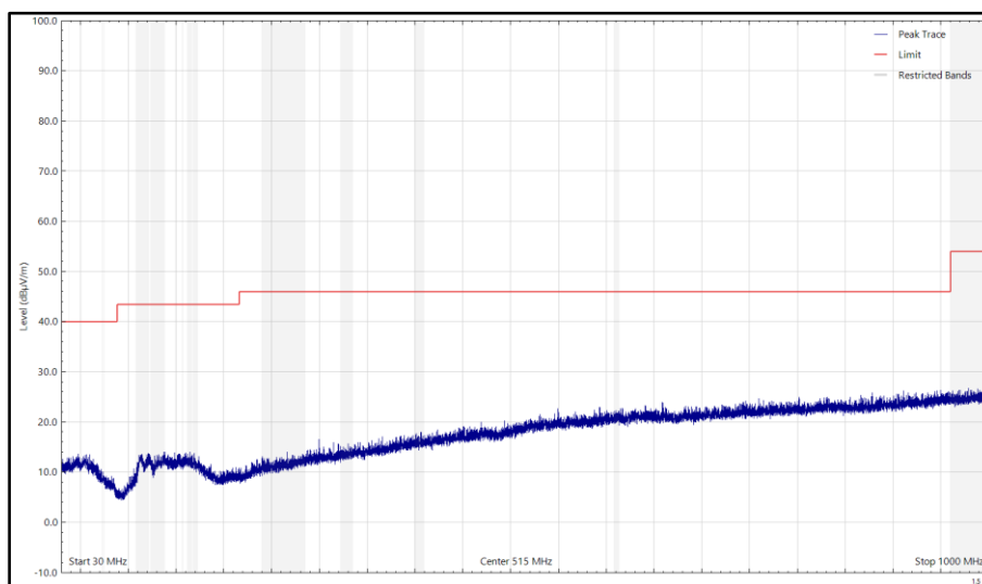
Figure 36 - CH18_LE1M_X Plane, 2442 MHz, 30 MHz to 1 GHz, Horizontal (Peak)
