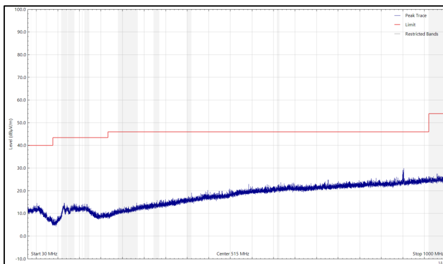
Figure 32 - CH37_LE1M_Z Plane, 2402 MHz, 30 MHz to 1 GHz, Horizontal (Peak)
