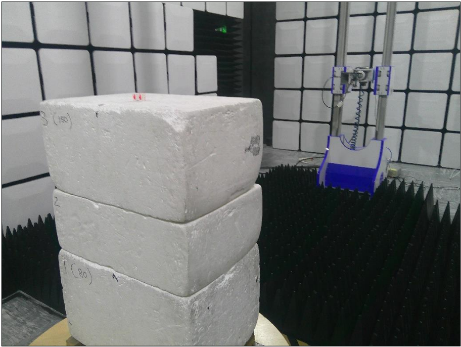
Figure 67 - Test Setup - 8 GHz to 18 GHz Y Plane
