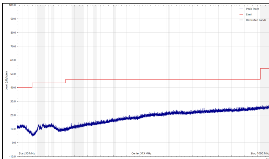
Figure 54 - CH39_LE1M_Y Plane, 2480 MHz, 30 MHz to 1 GHz, Horizontal (Peak)
