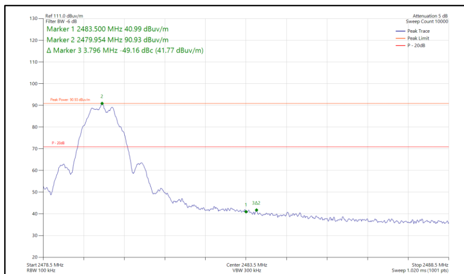
Figure 22 - CH39_UBE_LE1M_Core0_iPA, 2480 MHz, Band Edge Frequency 2483.5 MHz
