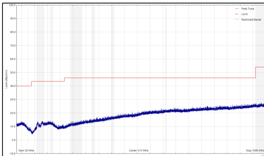
Figure 30 - CH37_LE1M_Y Plane, 2402 MHz, 30 MHz to 1 GHz, Horizontal (Peak)
