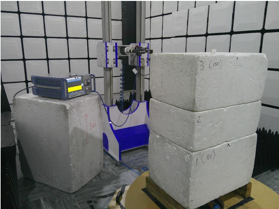
Figure 73 – 18 GHz to 25 GHz Y Plane
