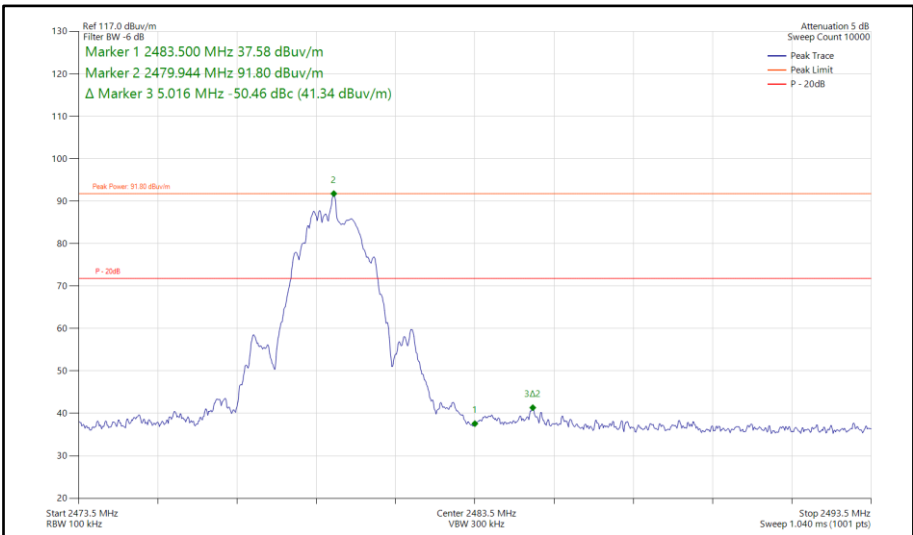
Figure 24 - CH39_UBE_LE1M_Core0_iPA, 2480 MHz, Band Edge Frequency 2483.5 MHz
