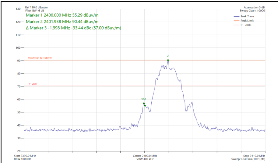
Figure 23 - CH37_LBE_LE1M_Core0_iPA, 2402 MHz, Band Edge Frequency 2400 MHz
