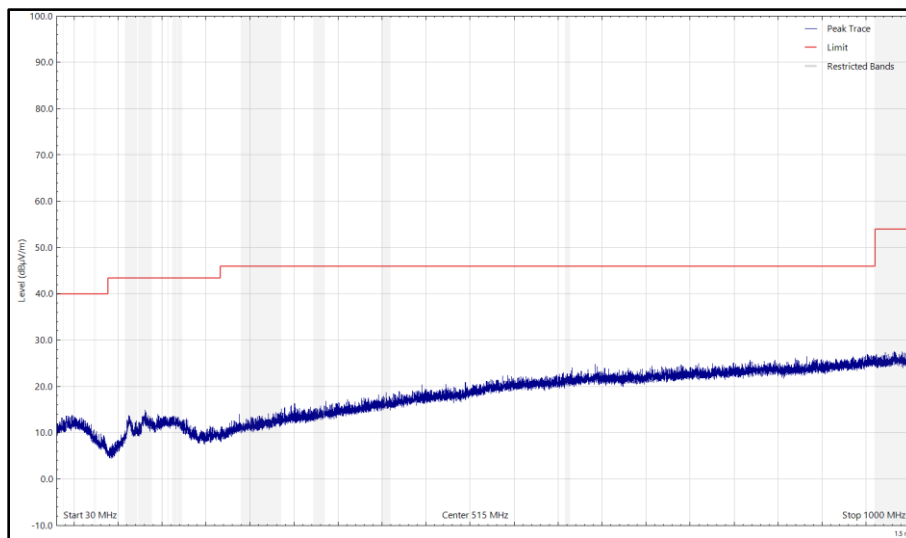
Figure 26 - CH37_LE1M_X Plane, 2402 MHz, 30 MHz to 1 GHz, Horizontal (Peak)
