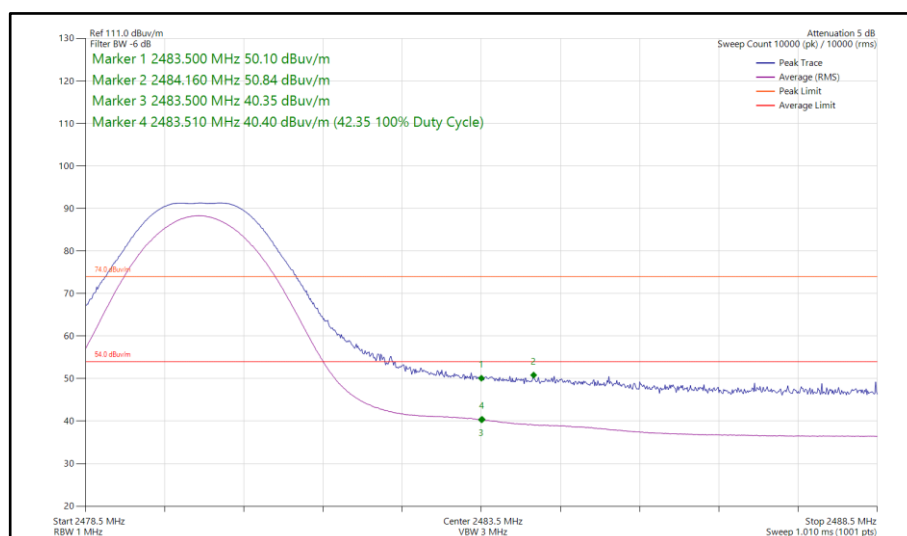
Figure 3 - CH39_URB_LE1M_Core0_iPA, 2480 MHz, Band Edge Frequency 2483.5 MHz
