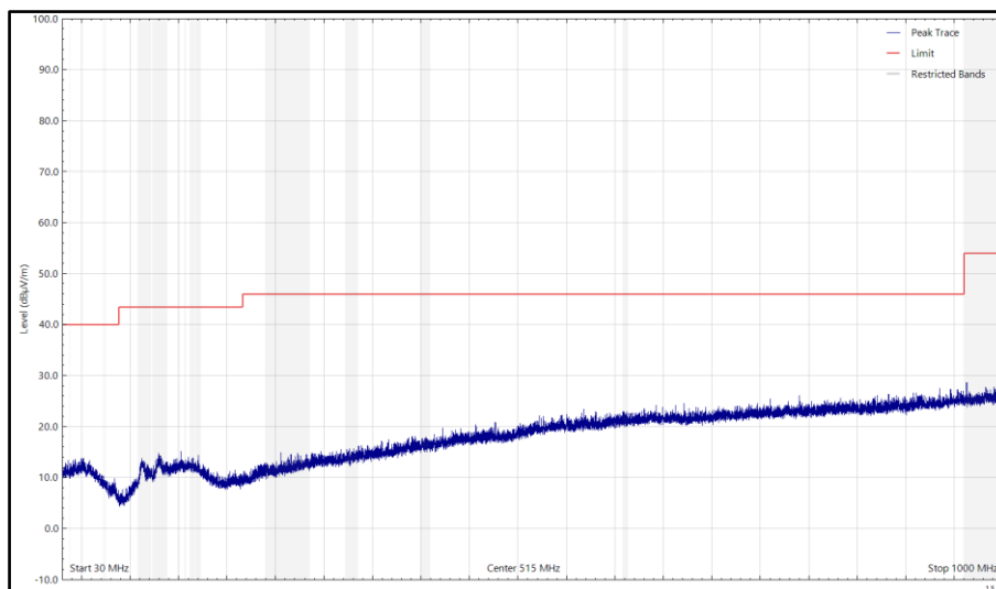
Figure 38 - CH18_LE1M_X Plane, 2442 MHz, 30 MHz to 1 GHz, Horizontal (Peak)
