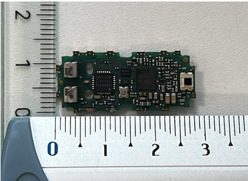
PCB Bottom side view
