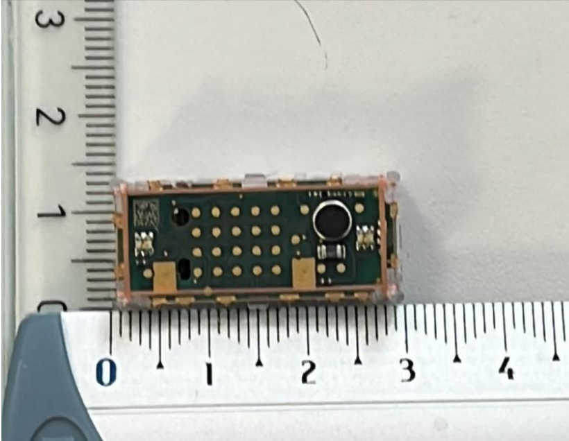
PCB Bottom side view
