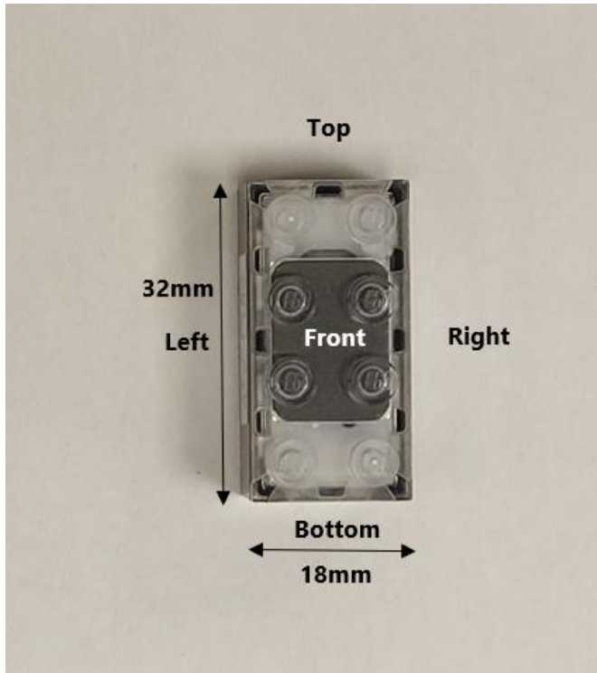
Figure 8 Dimensions of the DUT
