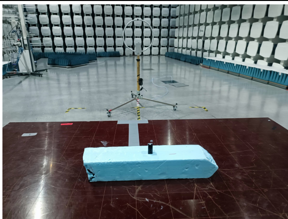
Radiated Emissions 9 kHz – 30 MHz
