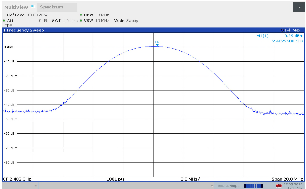
Conducted Power , Ch2402MHz
