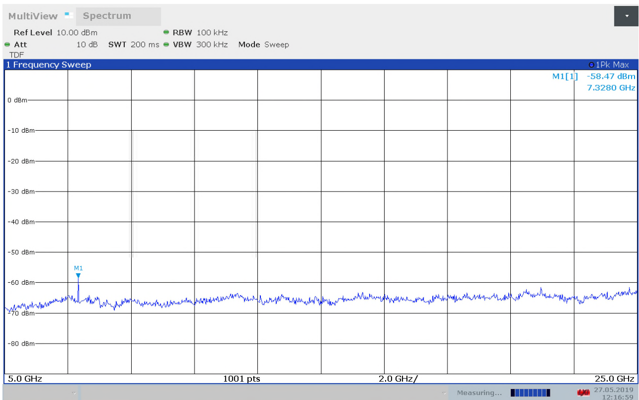
Conducted spurious emissions, 5GHz - 25GHz, ch2440MHz
