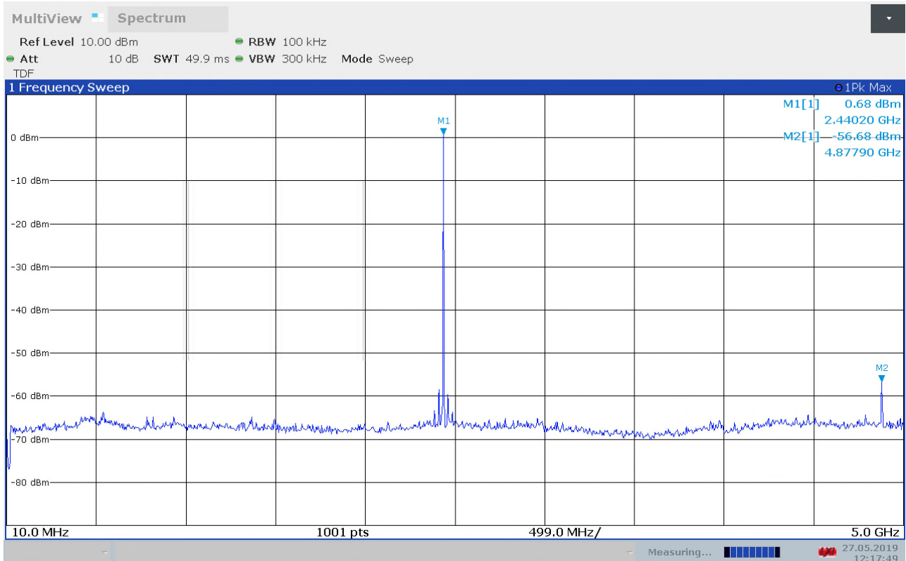
Conducted spurious emissions, 10MHz - 5GHz, ch2440MHz
