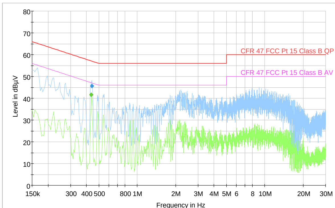
Full Spectrum
