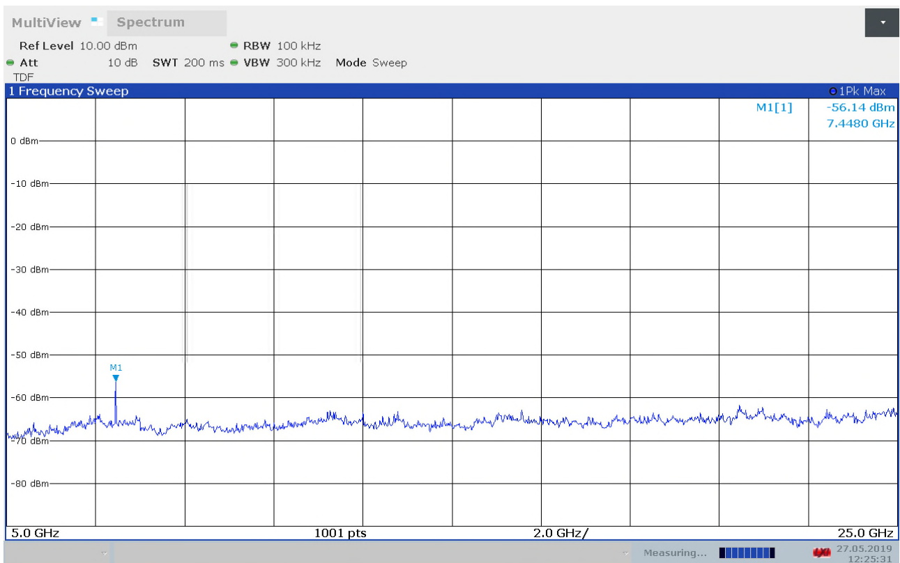
Conducted spurious emissions, 5GHz - 25GHz, ch2480MHz
