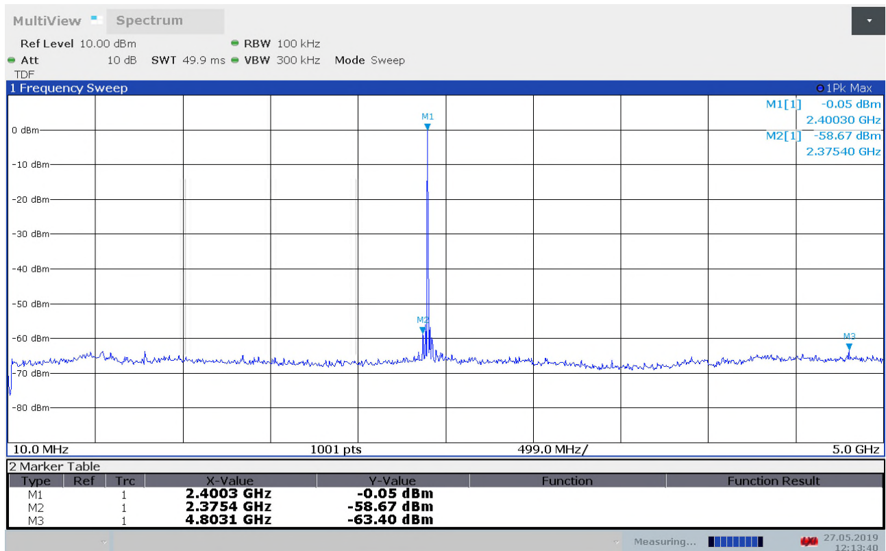
Conducted spurious emissions, 10MHz - 5GHz, ch2402MHz
