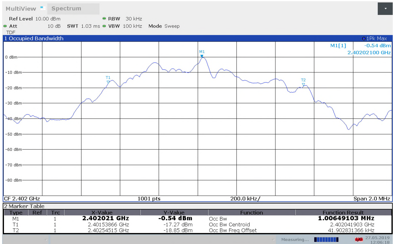
99% Bandwidth , ch2402MHz
