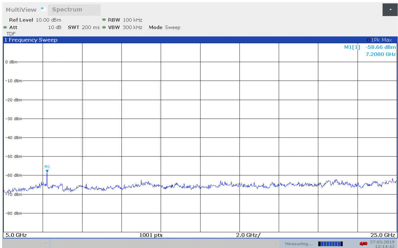
Conducted spurious emissions, 5GHz - 25GHz, ch2402MHz
