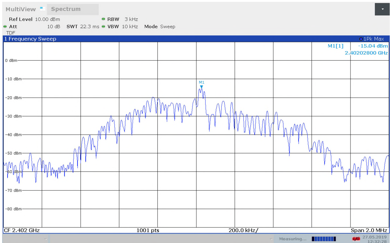
Conducted PSD, ch2402MHz
