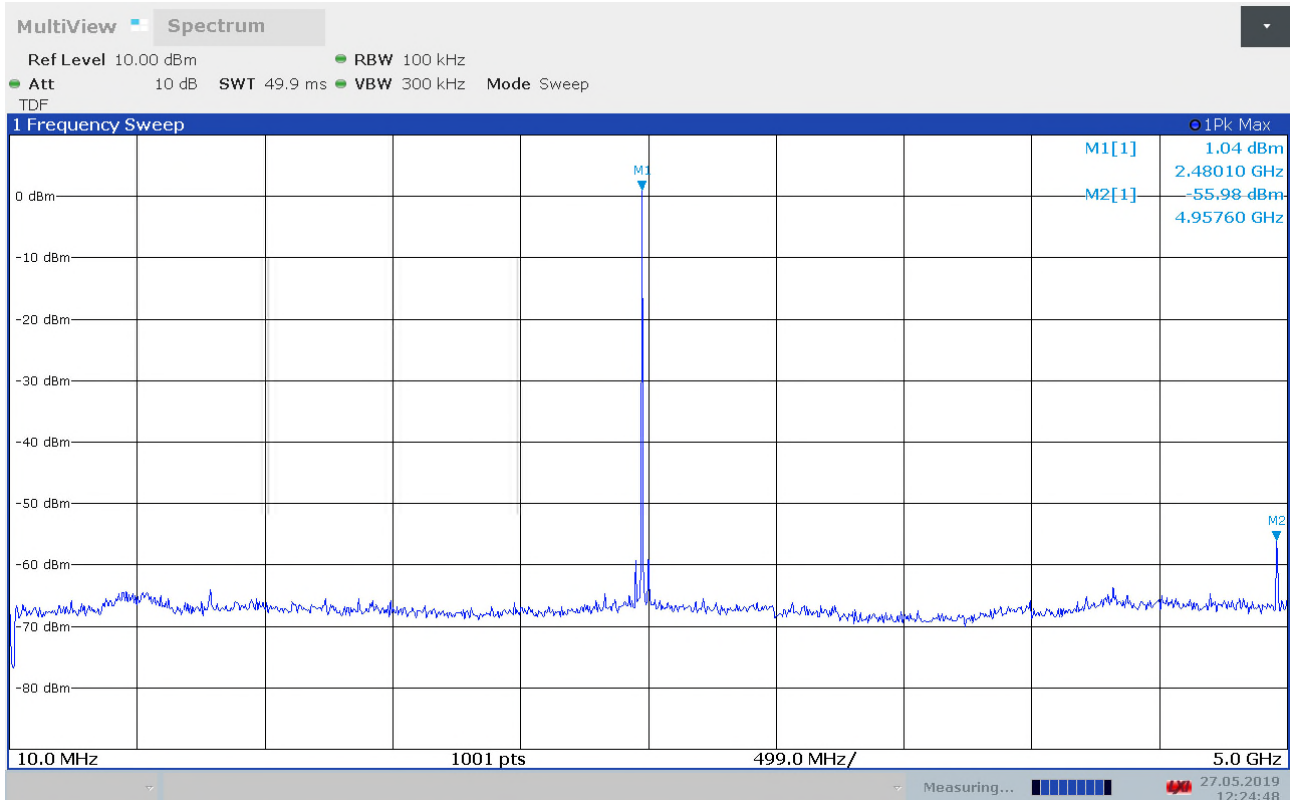
Conducted spurious emissions, 10MHz - 5GHz, ch2480MHz
