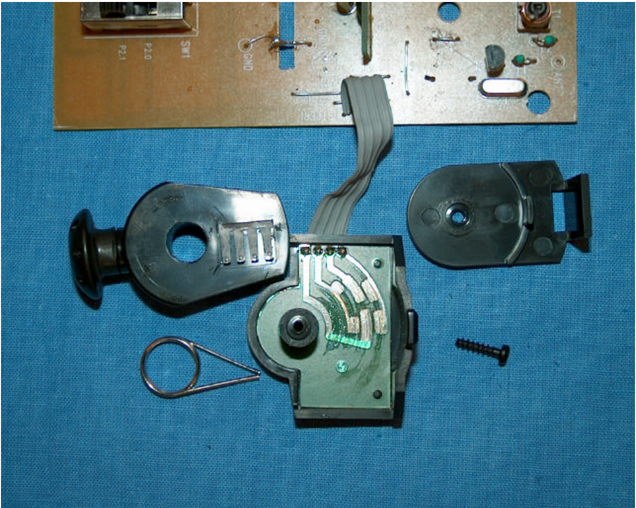
Steering control (additional PCB)
