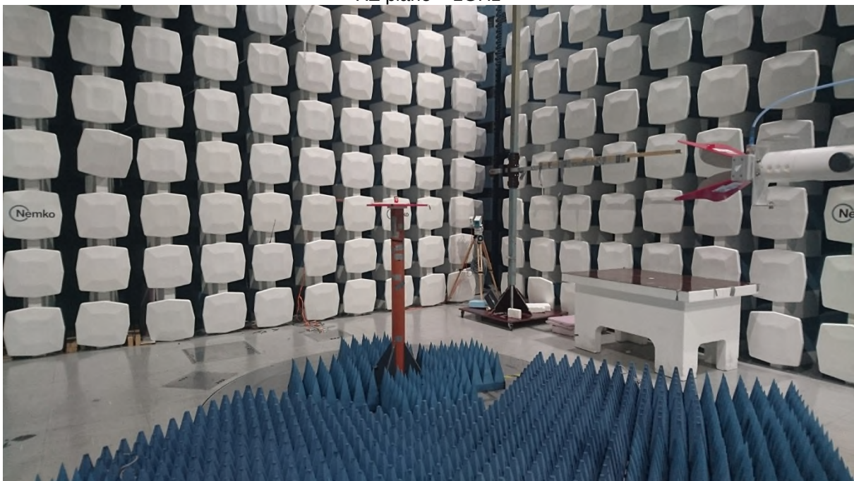
Radiated emissions > 1GHz
