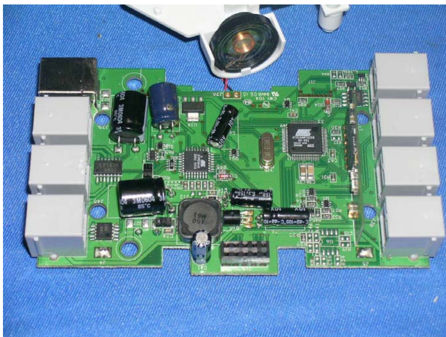
Main Unit's PCB comp side (View 1)
