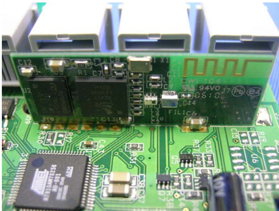
Main Unit's PCB comp side (View 2)
