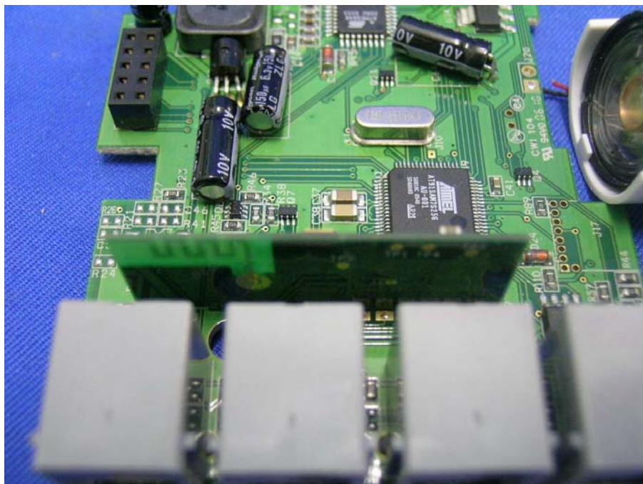
Main Unit's PCB comp side (View 3)
