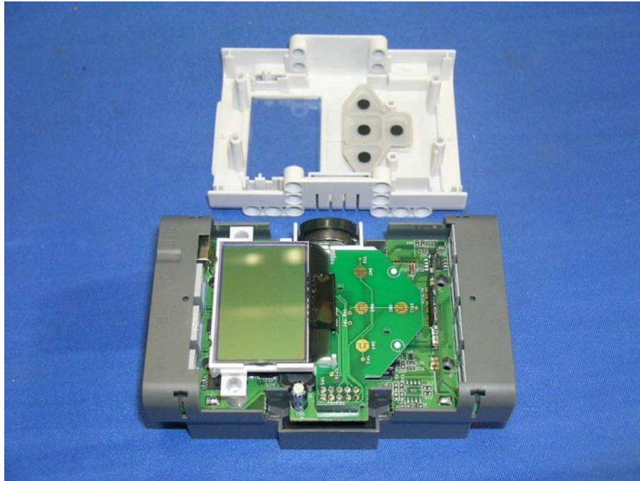
Main Unit assembly (View 1)
