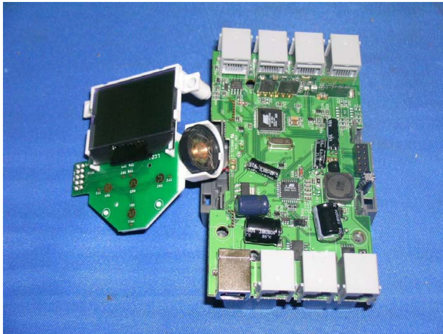
Main Unit assembly (View 2)
