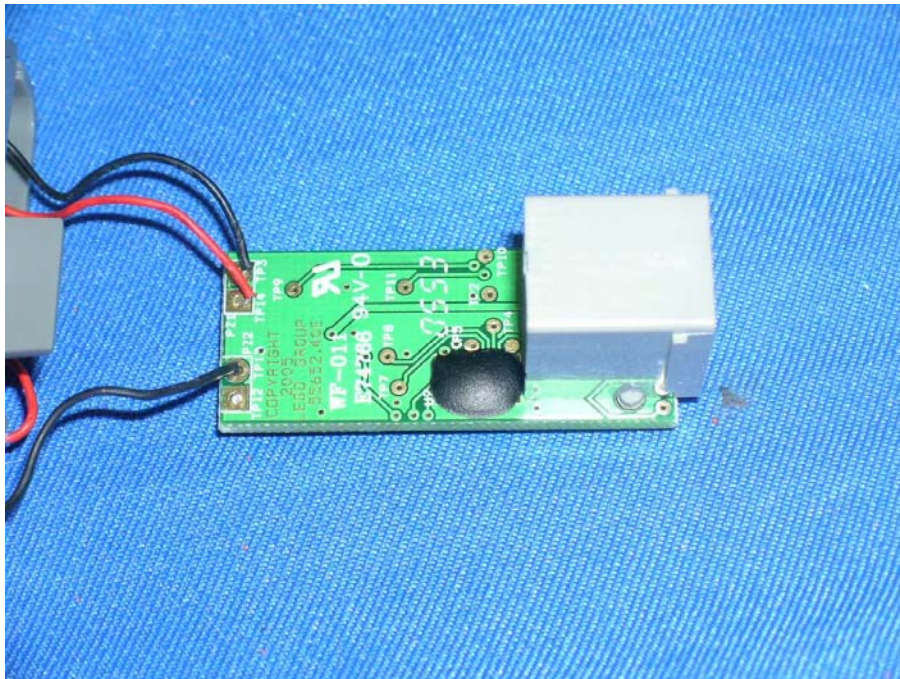
Ultrasonic sensor PCB comp side
