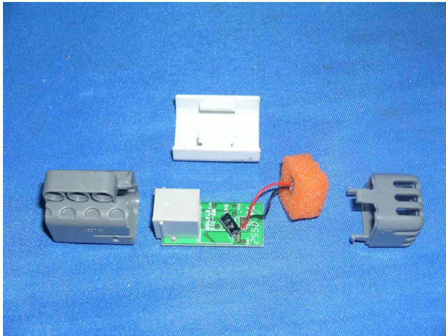
Microphone assembly
