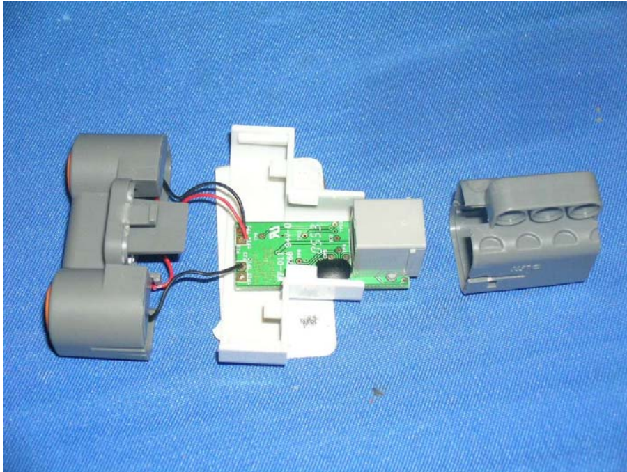
Ultrasonic sensor assembly
