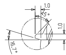
SCALE 5:1 DETAIL C
