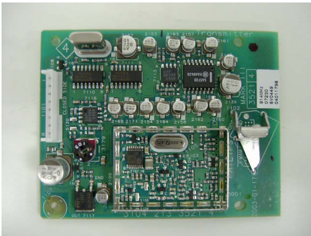
Component side without shield
