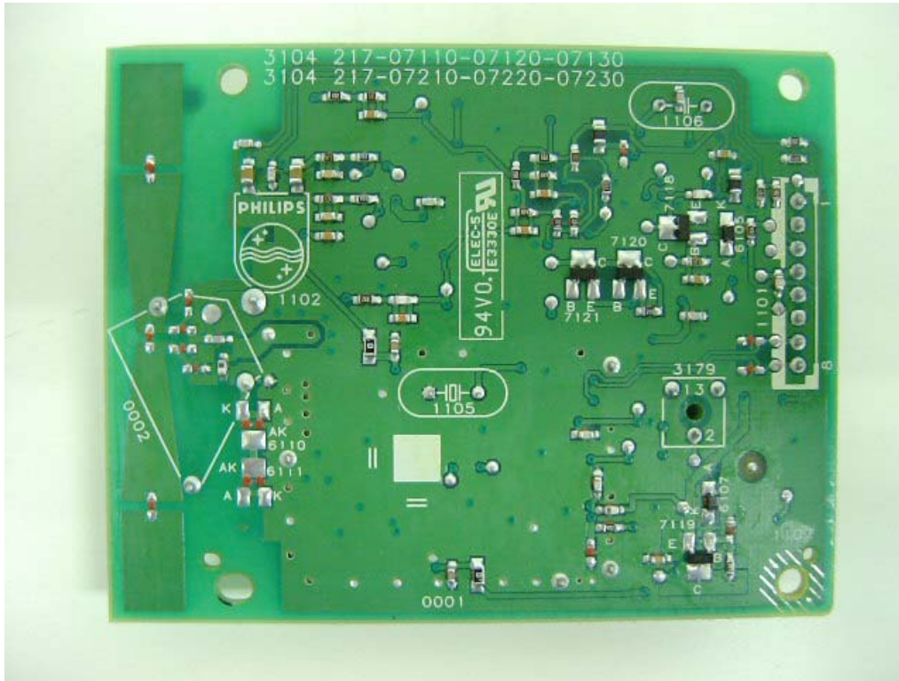
Solder side
