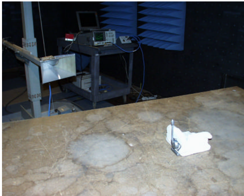
Harmonics and Spurious Emission
