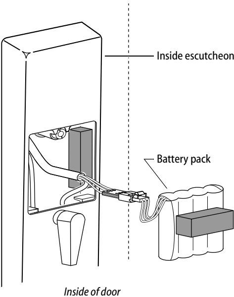
Figure 14 Connecting the battery pack
