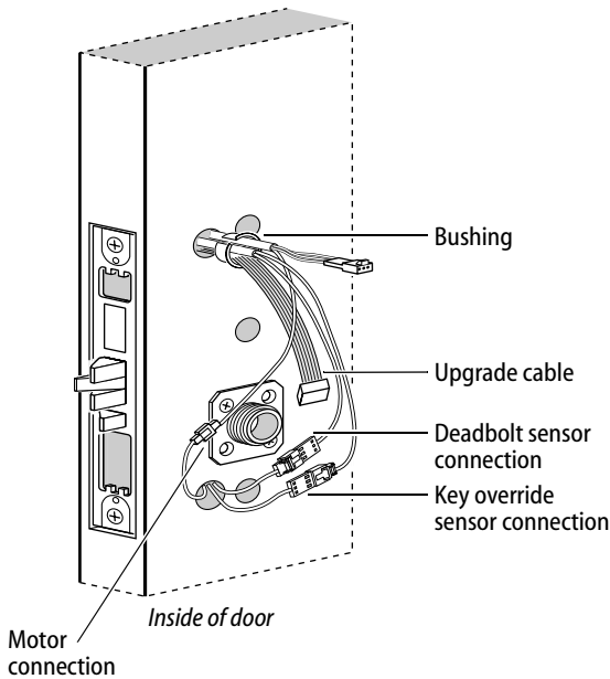
Figure 12 Making the motor connection and sensor connections
