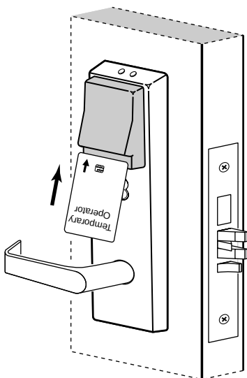
Figure 19b Using the temporary operator card with a smart card reader
