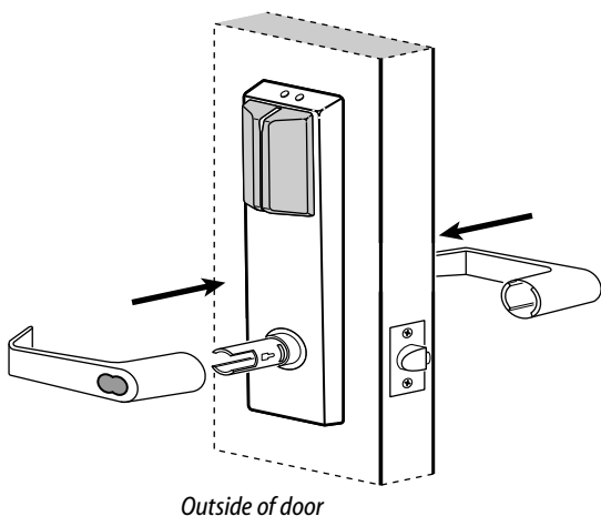
Figure 15 Installing the levers
