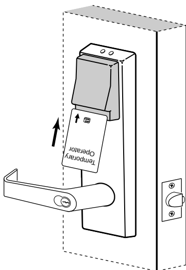
Figure 18b Using the temporary operator card with a smart card reader
