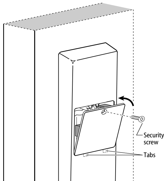
Figure 17 Installing the access door
