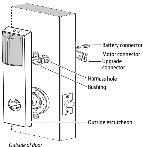
Figure 11 Feeding the wire harness connectors through the harness hole
