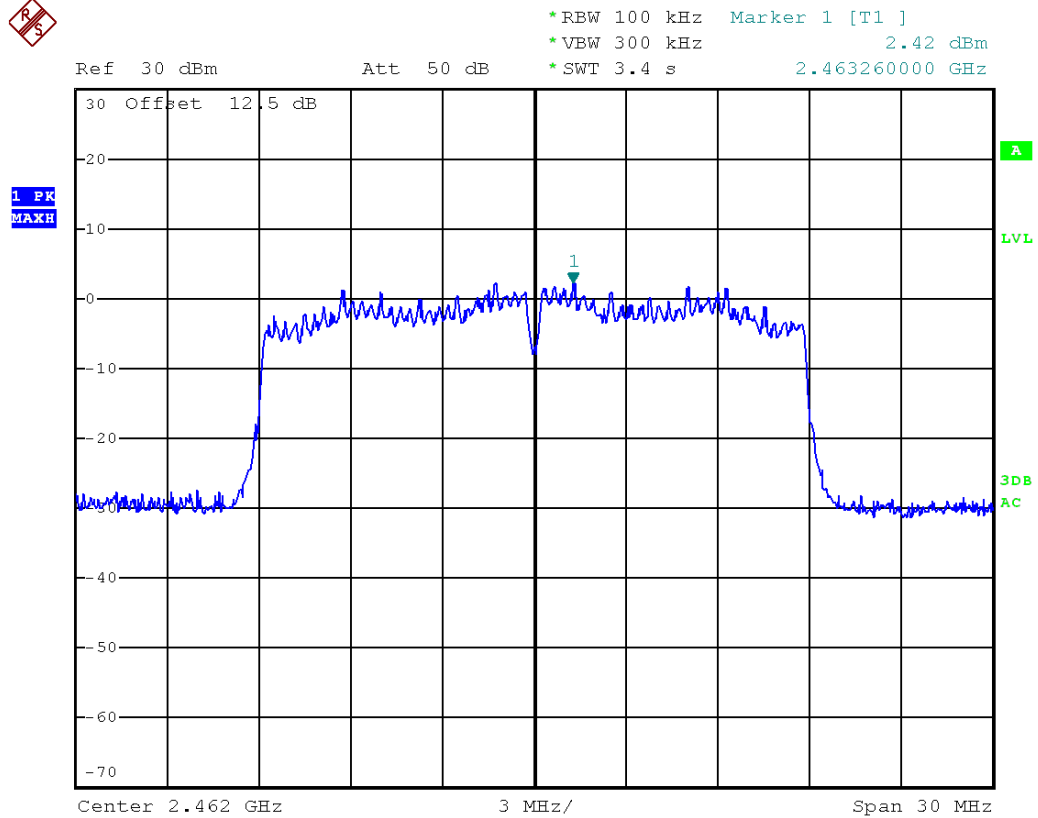
Channel 2462MHz
