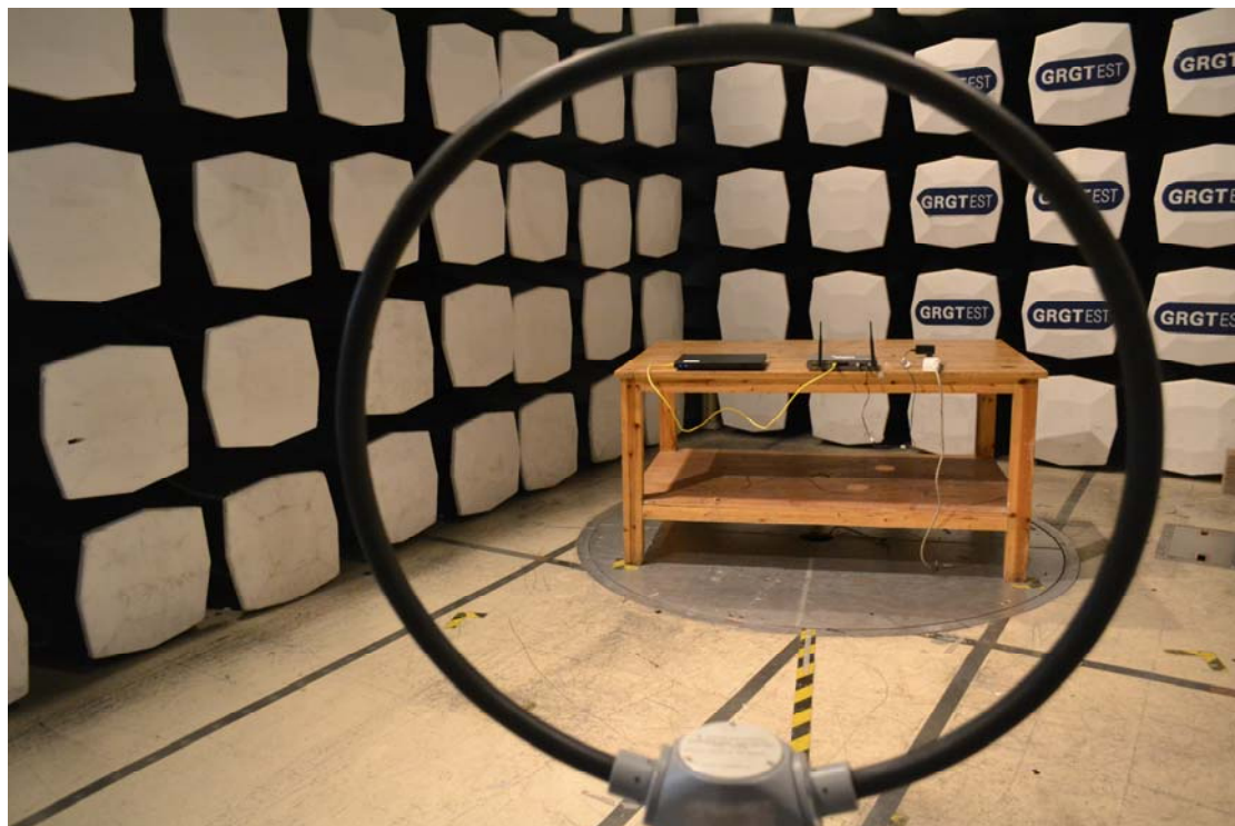
RSE (9K-30M)
