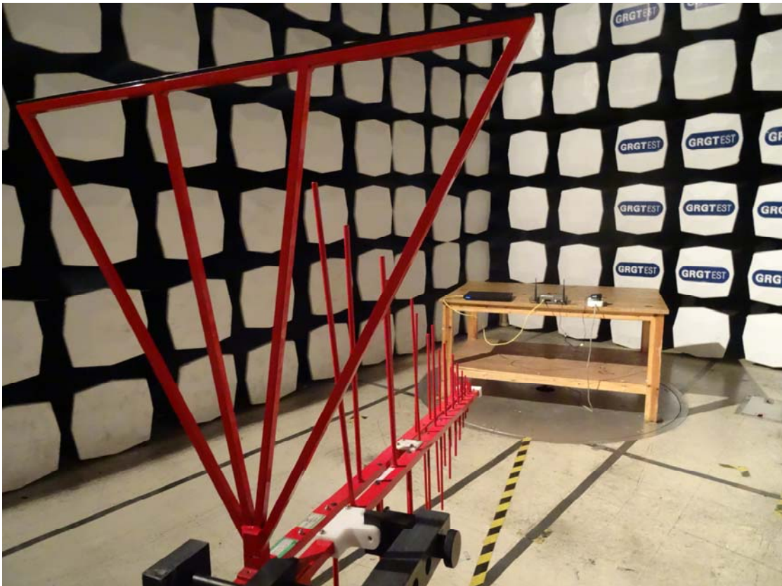
RSE (30M-1G)
