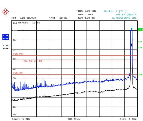
Bandedge
