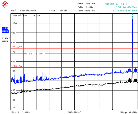
Bandedge
