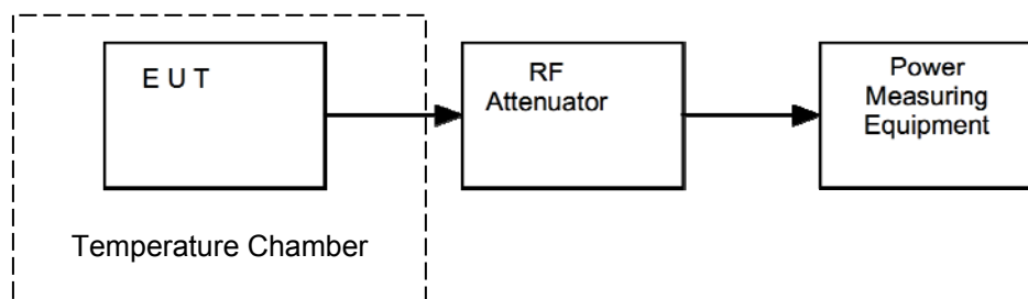
Figure vii Test Setup
