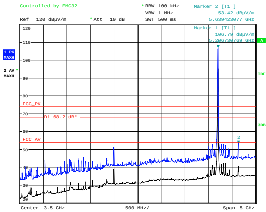
Bandedge
