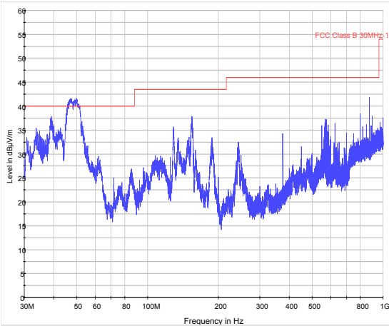
30 MHz – 1 GHz
