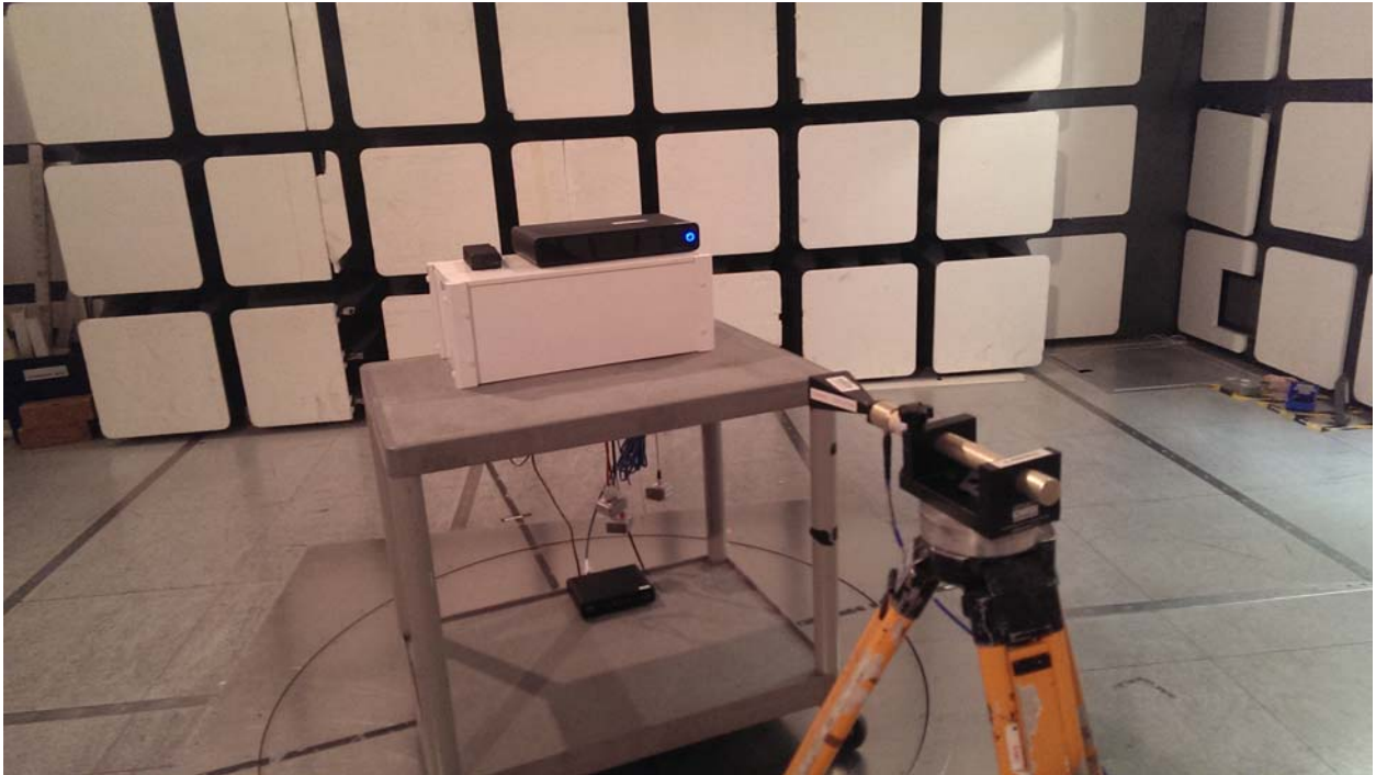
Radiated Emissions 18-30GHz
