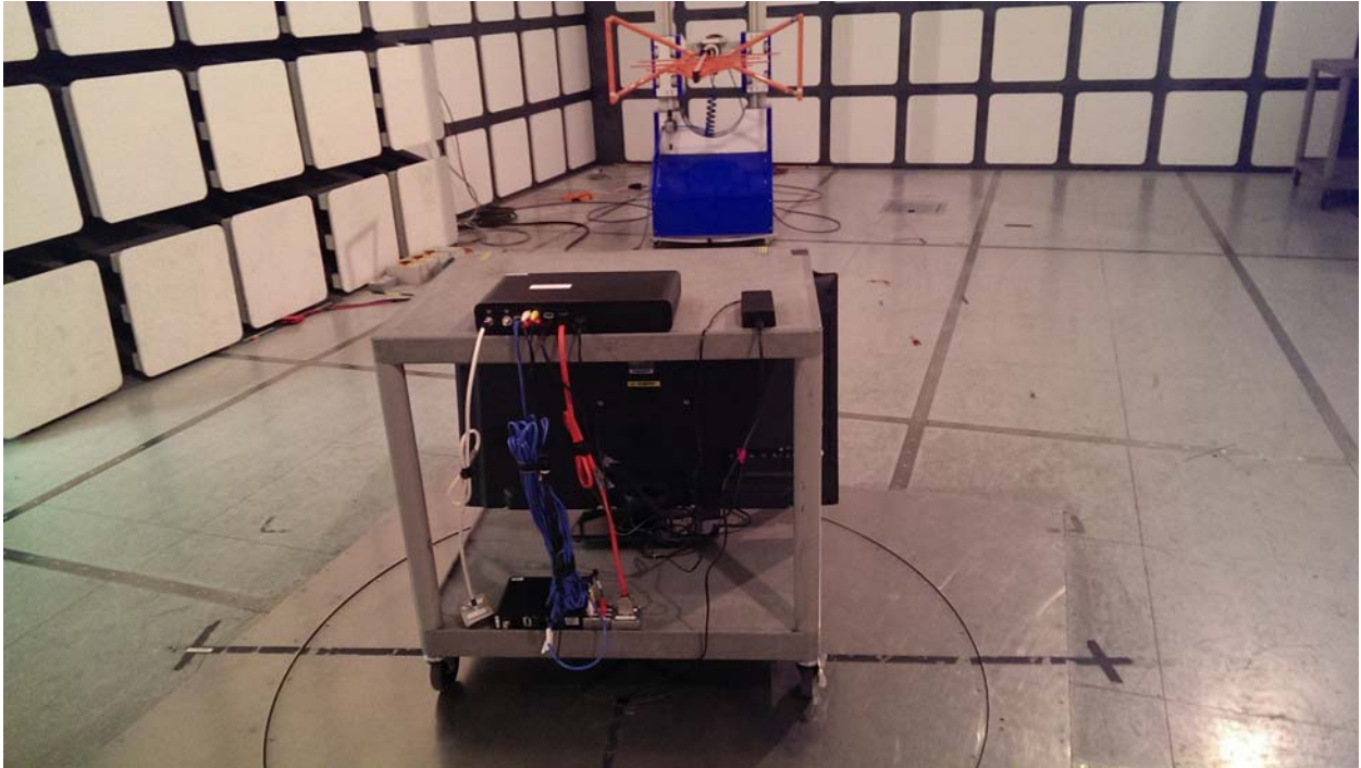
Radiated Emissions 30MHz-1GHz
