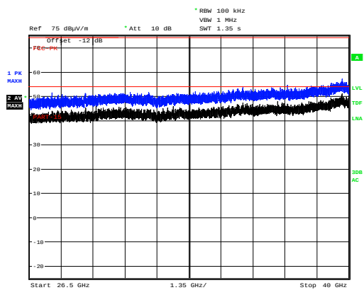
26.5 GHz – 40 GHz
