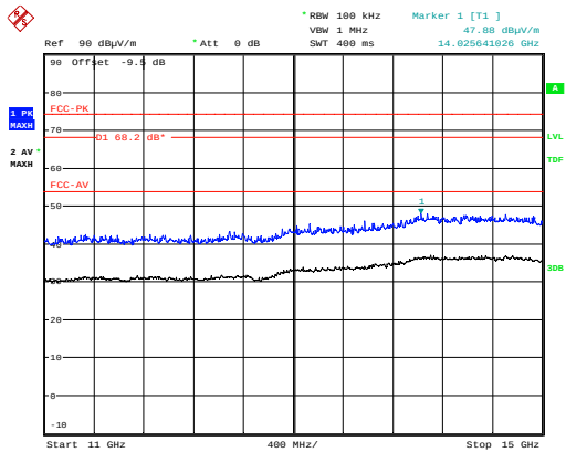
11 GHz – 15 GHz
