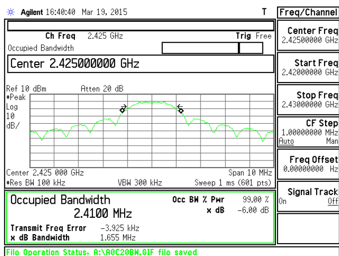
Antenna 0 2425.0 MHz
