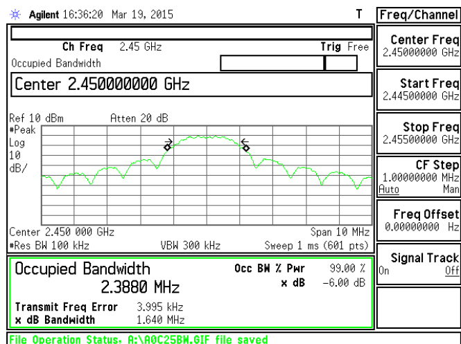
Antenna 0 2450.0 MHz
