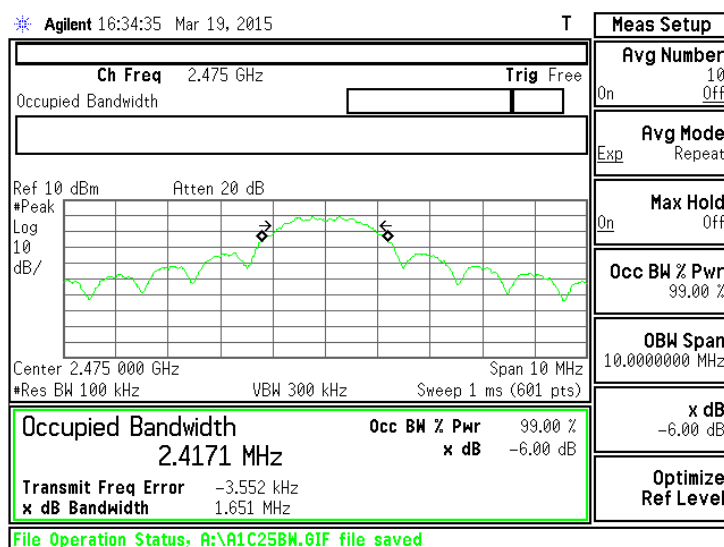
Antenna 0 2475.0 MHz
