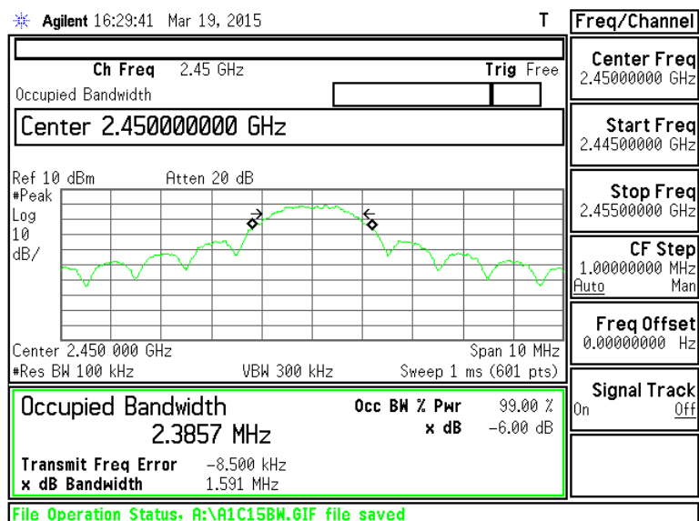
Antenna 1 2450.0 MHz
