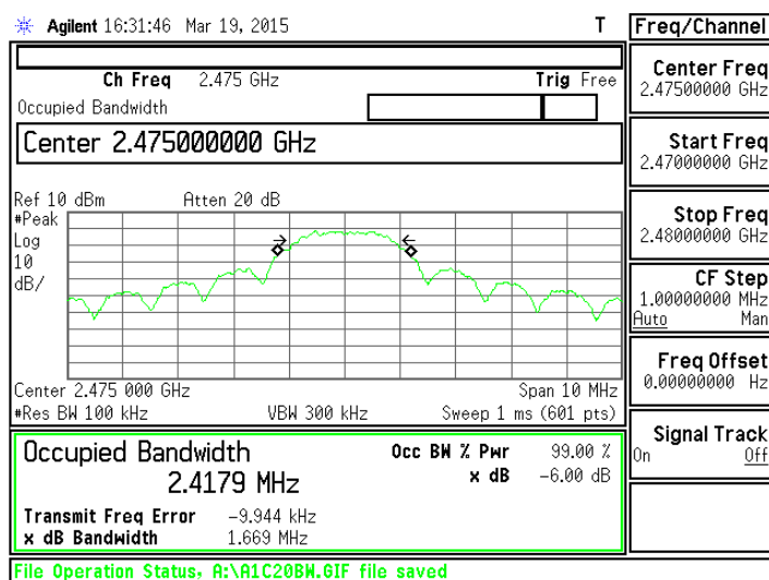
Antenna 1 2475.0 MHz
