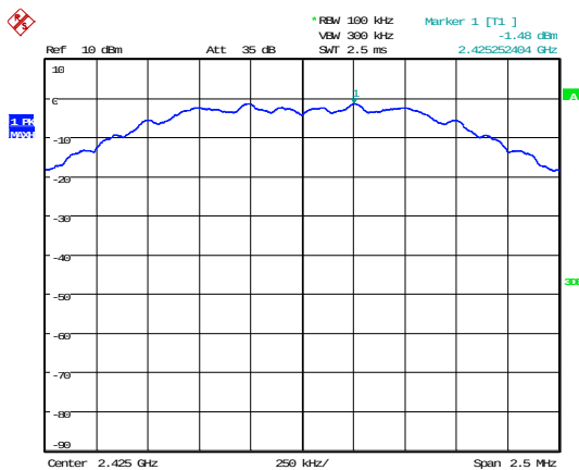
Antenna 1 2425.0 MHz
