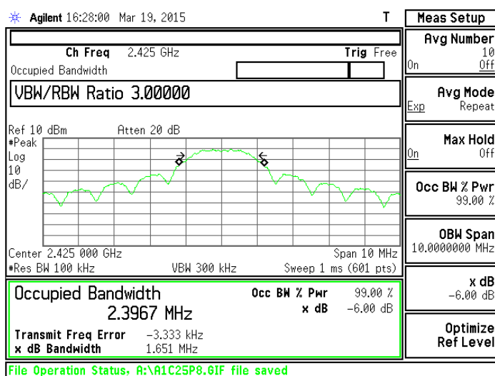
Antenna 1 2425.0 MHz
