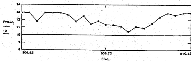
Process Gain by Frequency (in Mhz)
