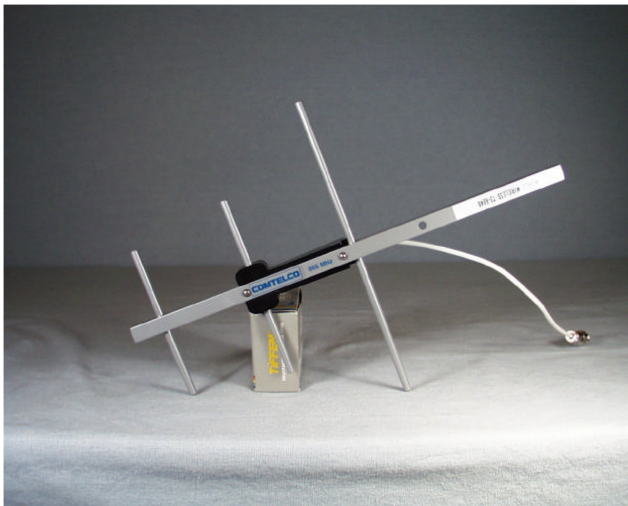
Comtelco Model Y2283A-66 Yagi Antenna
