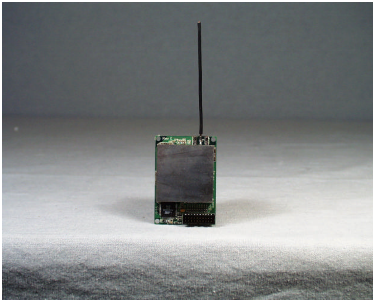
Back View of the 900 \mu Hopper (Dipole Antenna)
