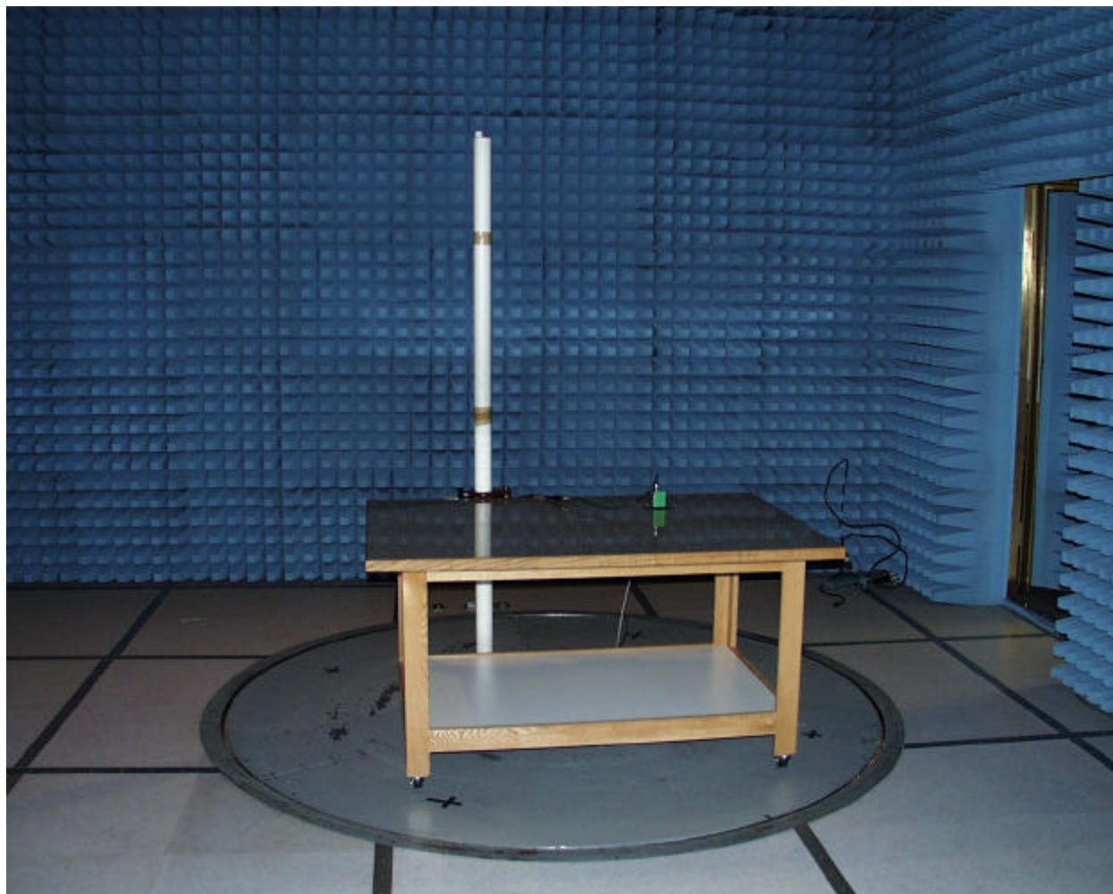
Worst case radiated emissions (Omni antenna)
