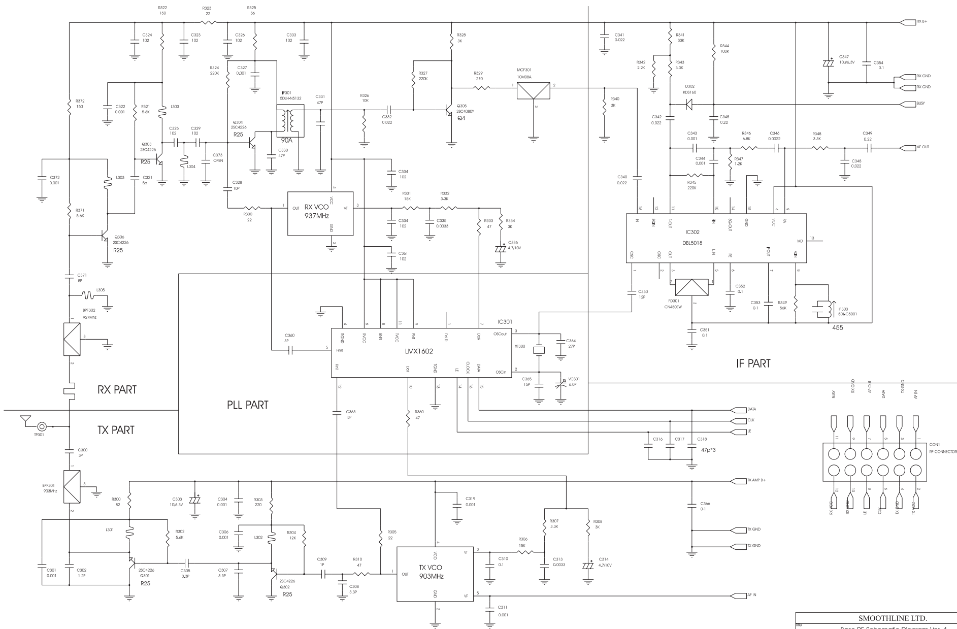
Base RF Schematic Diagram
