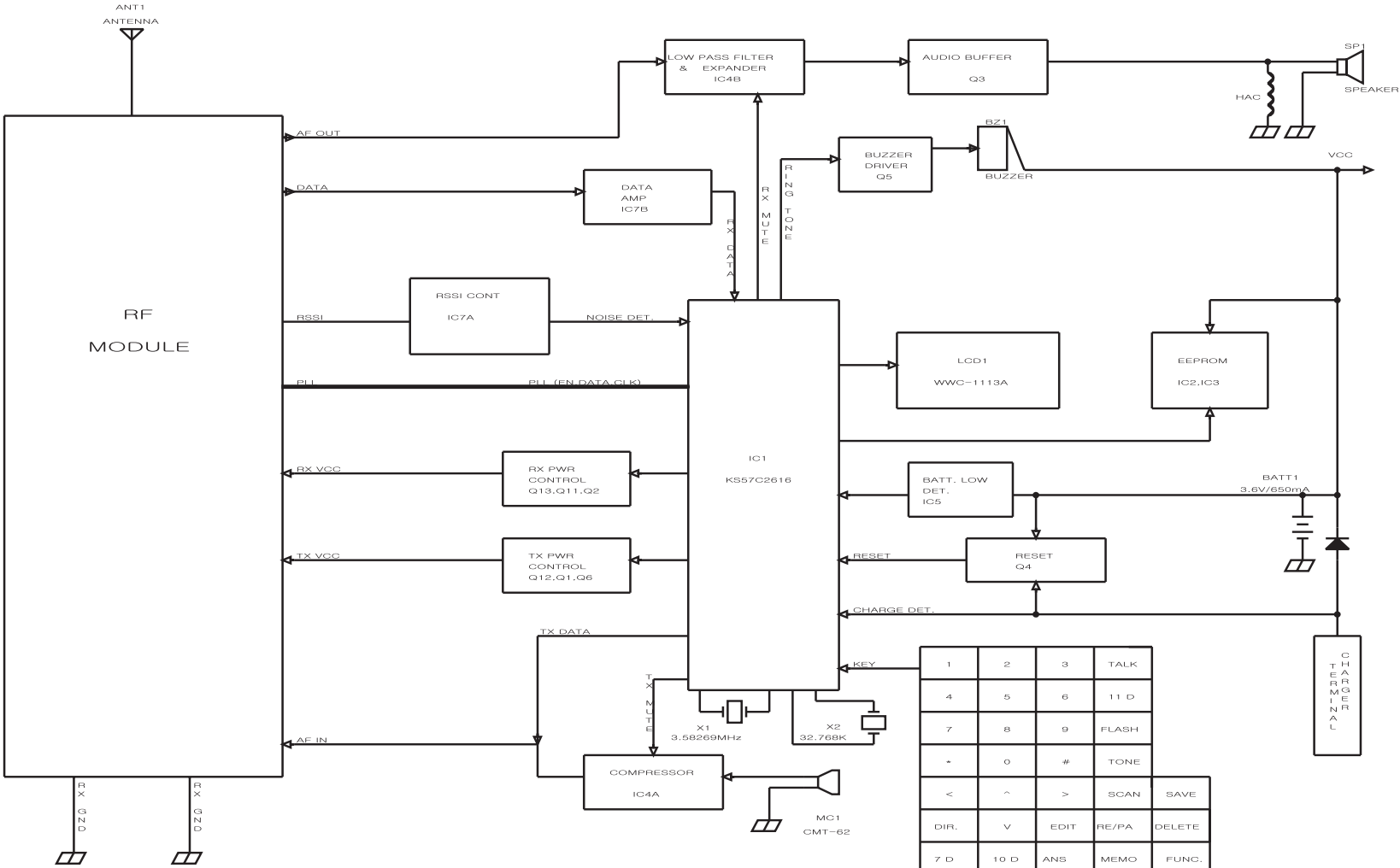
MH-9932 V4 HAND SET BLOCK DIAGRAM
