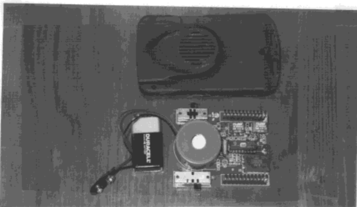
5. FCC ID: NQW267-26 Top of board, enclosure and battery
