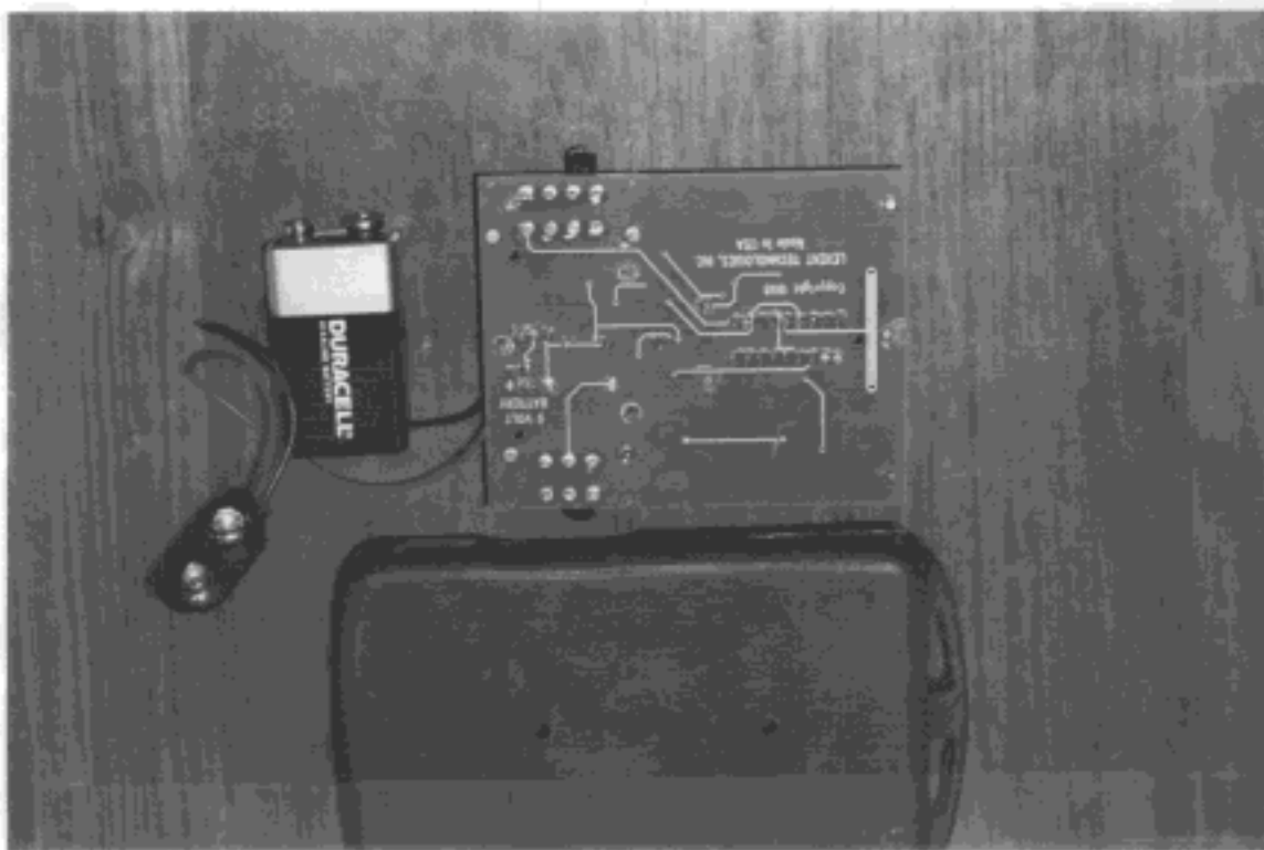
7. FCC ID: NQW267-26 Bottom of board, enclosure and battery
