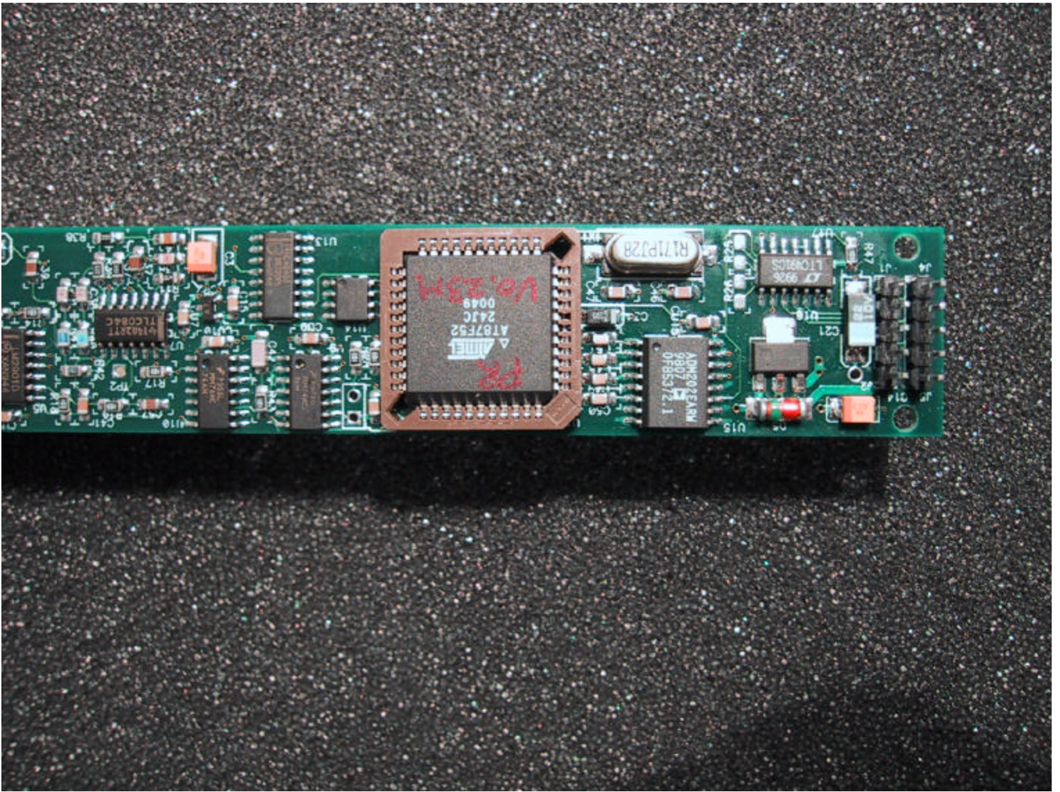
PCB TOP C
