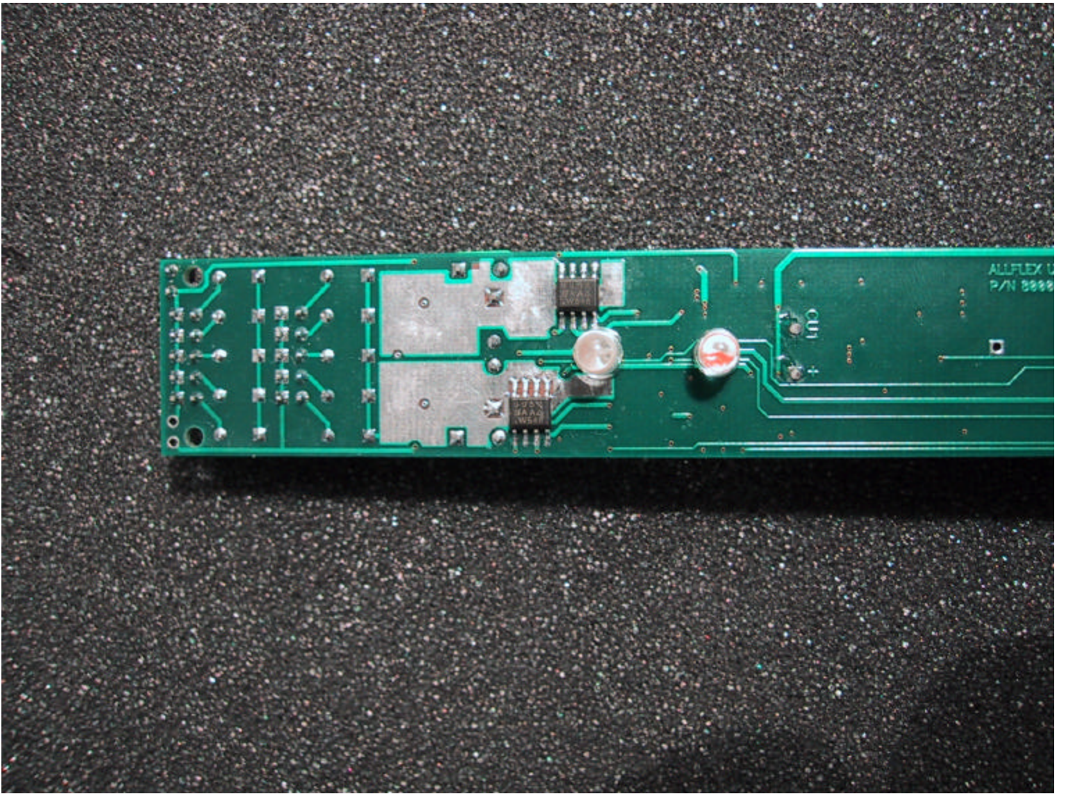
PCB BOTTOM A
