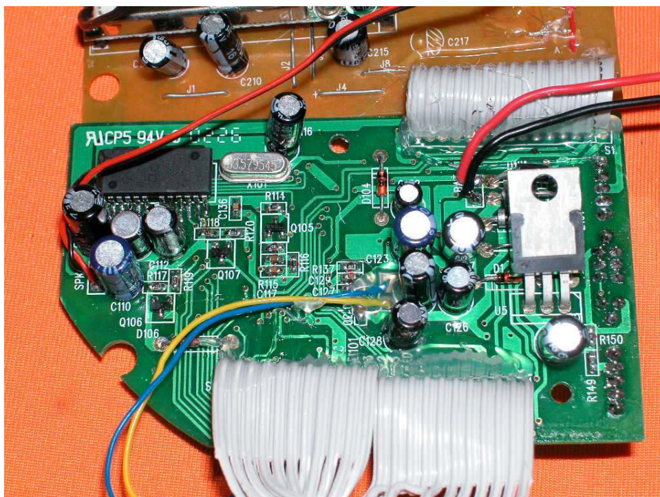
Base Another PCB comp side
