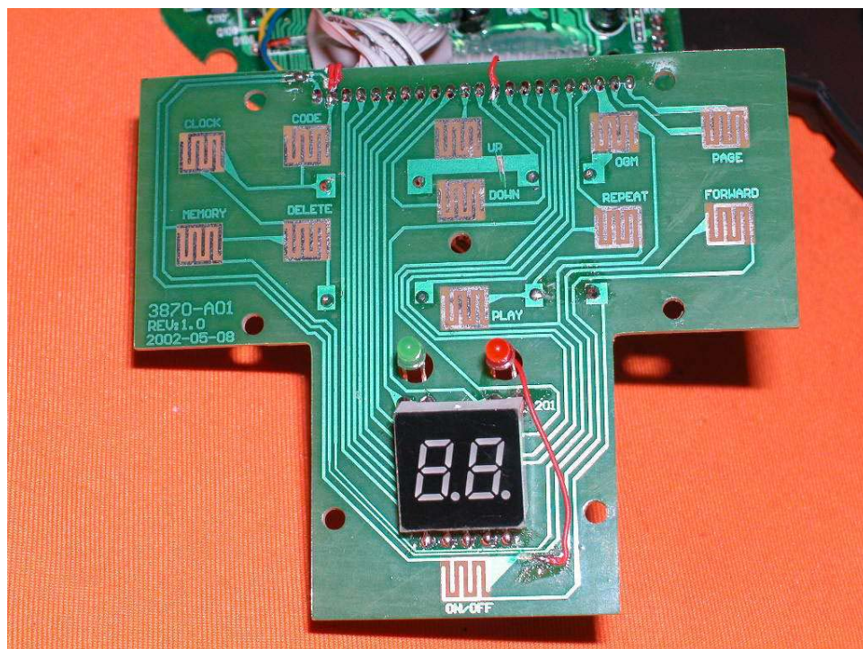
Base DAM PCB keypad side
