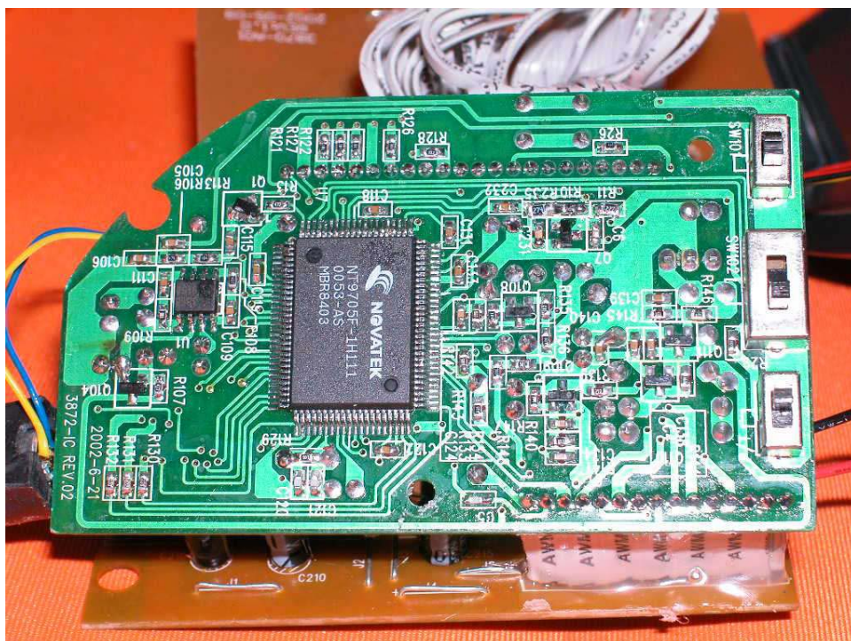
Base Another PCB solder side
