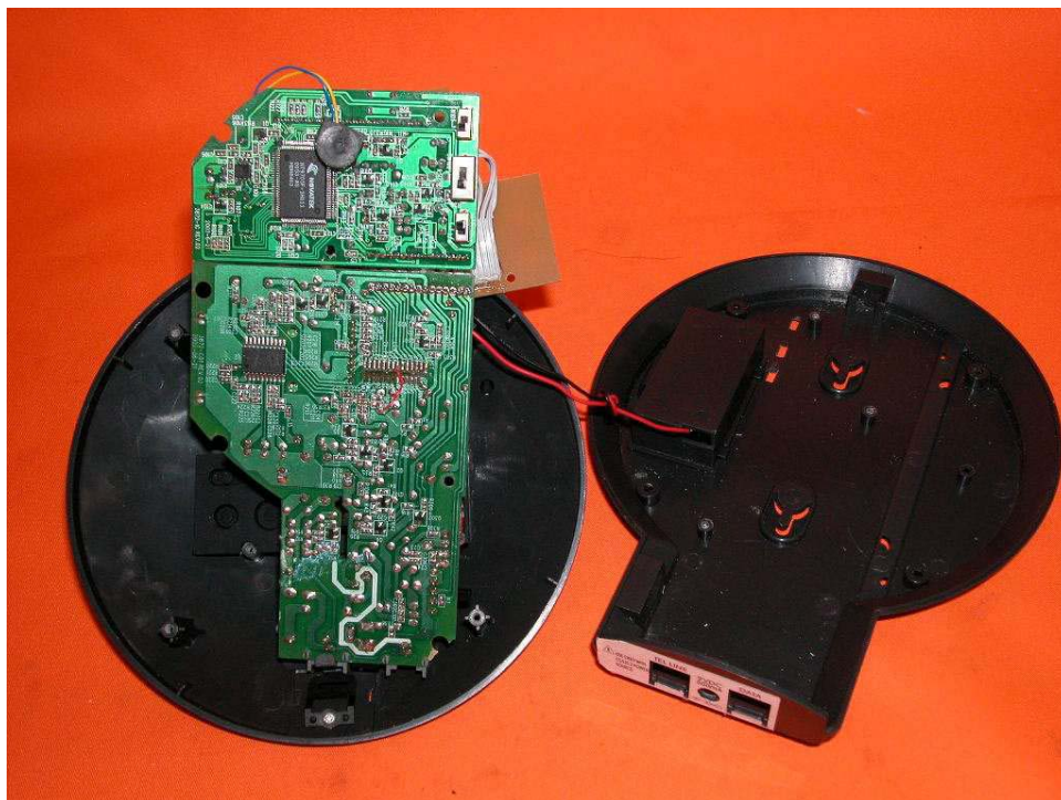
Base assembly (View 3)
