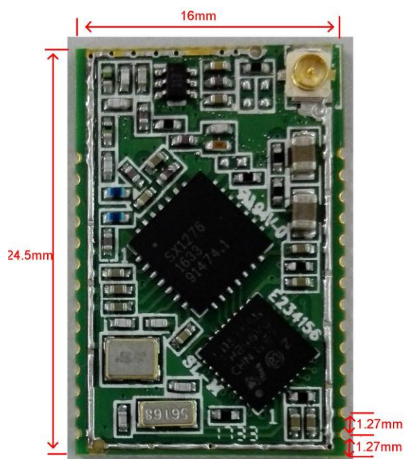
Figure 4 Mechanical Drawing and Dimensions
