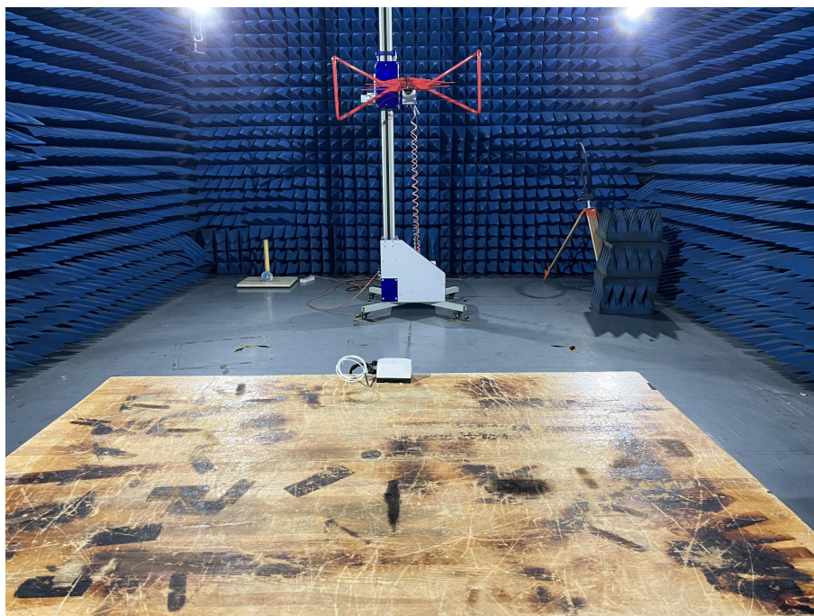
RE TEST SETUP (30M-1G)
