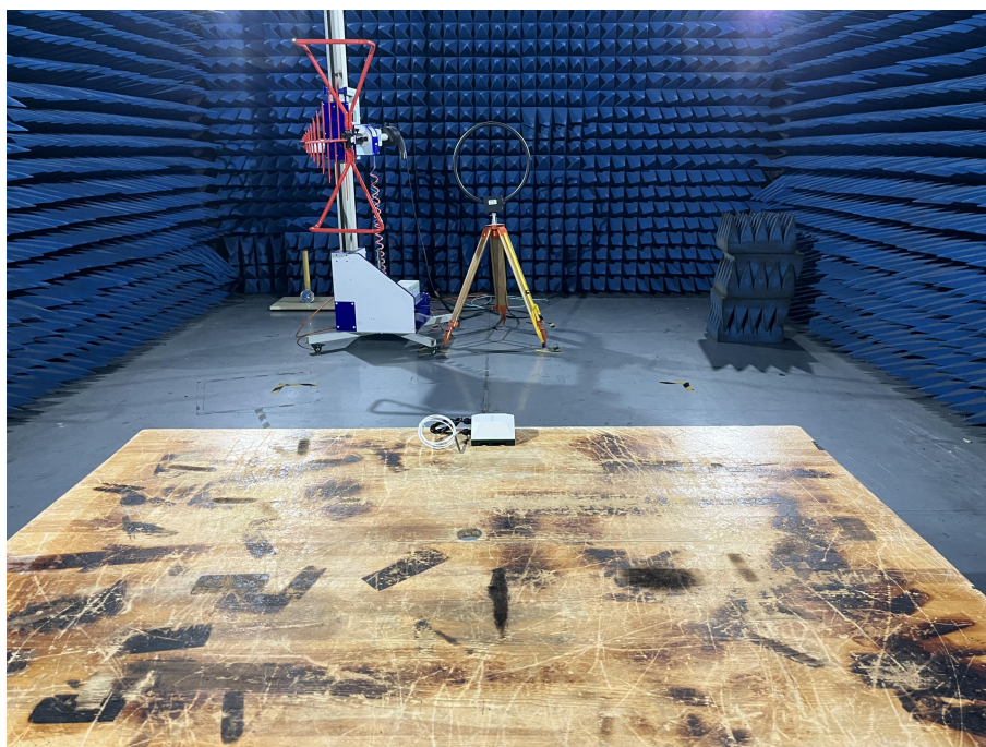
RE TEST SETUP (9k-30M)
