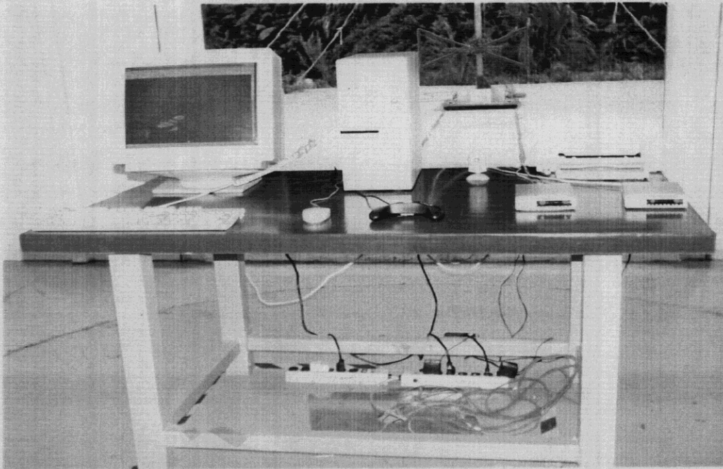
Back View of Radiated Emission Test (Mode 1)
