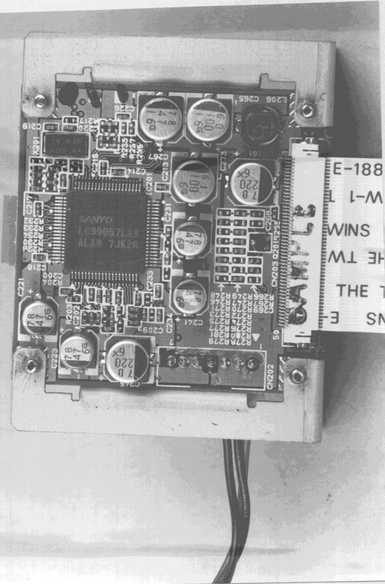
Photograph of the EUT Construction
