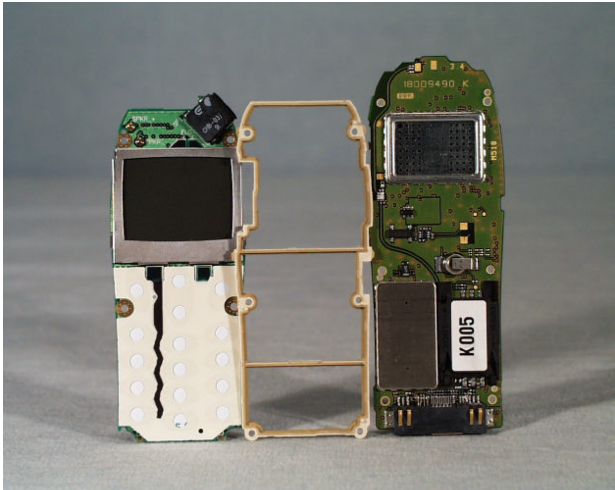
Back view of the MMI module, main PCB and RF gasket that is placed between the two boards
