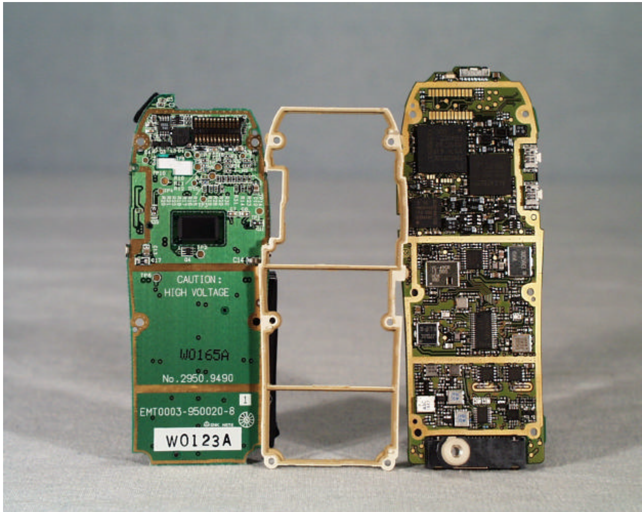
Front view of the MMI module, main PCB and RF gasket that is placed between the two boards
