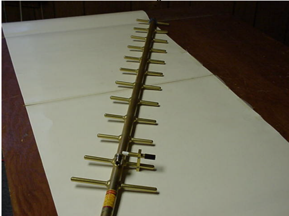
11 dBi Yagi
