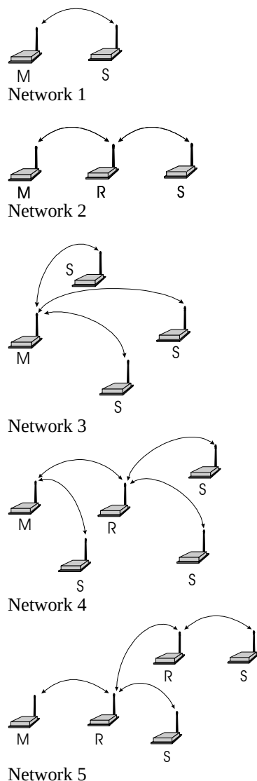
Figure 2 - Sample Network Topologies. Virtually any Combination of Slaves and Repeaters May be Used.
