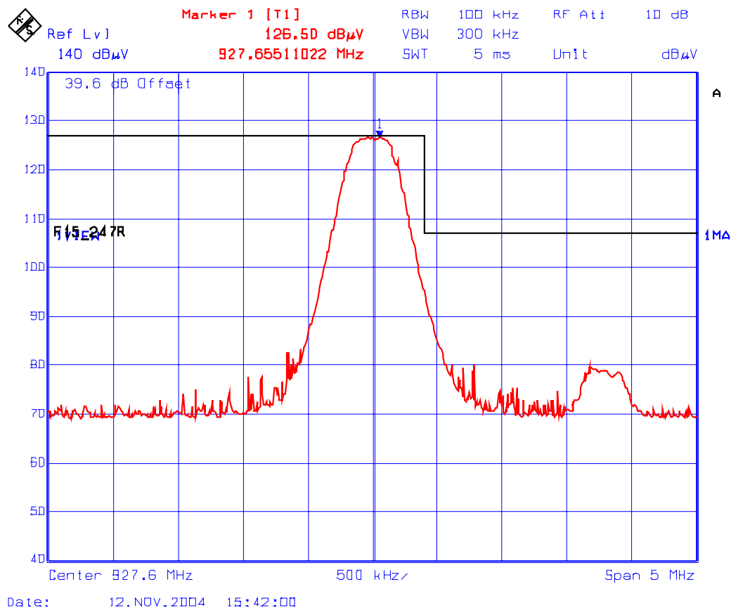
Plot 38: Band-Edge RF Radiated Emissions @ 3 meters Upper End of Frequency Band Test Configuration 1: EUT with ¼ Wave Antenna (1.5 dBi Gain) Rx Antenna Orientation: Vertical
