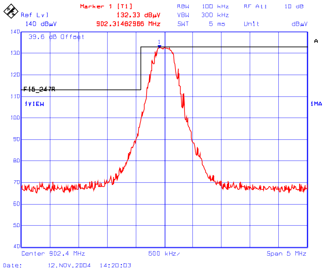
Plot 40: Band-Edge RF Radiated Emissions @ 3 meters Low End of Frequency Band Test Configuration 2: EUT with Rubber Duck Antenna (2 dBi Gain) Rx Antenna Orientation: Vertical
