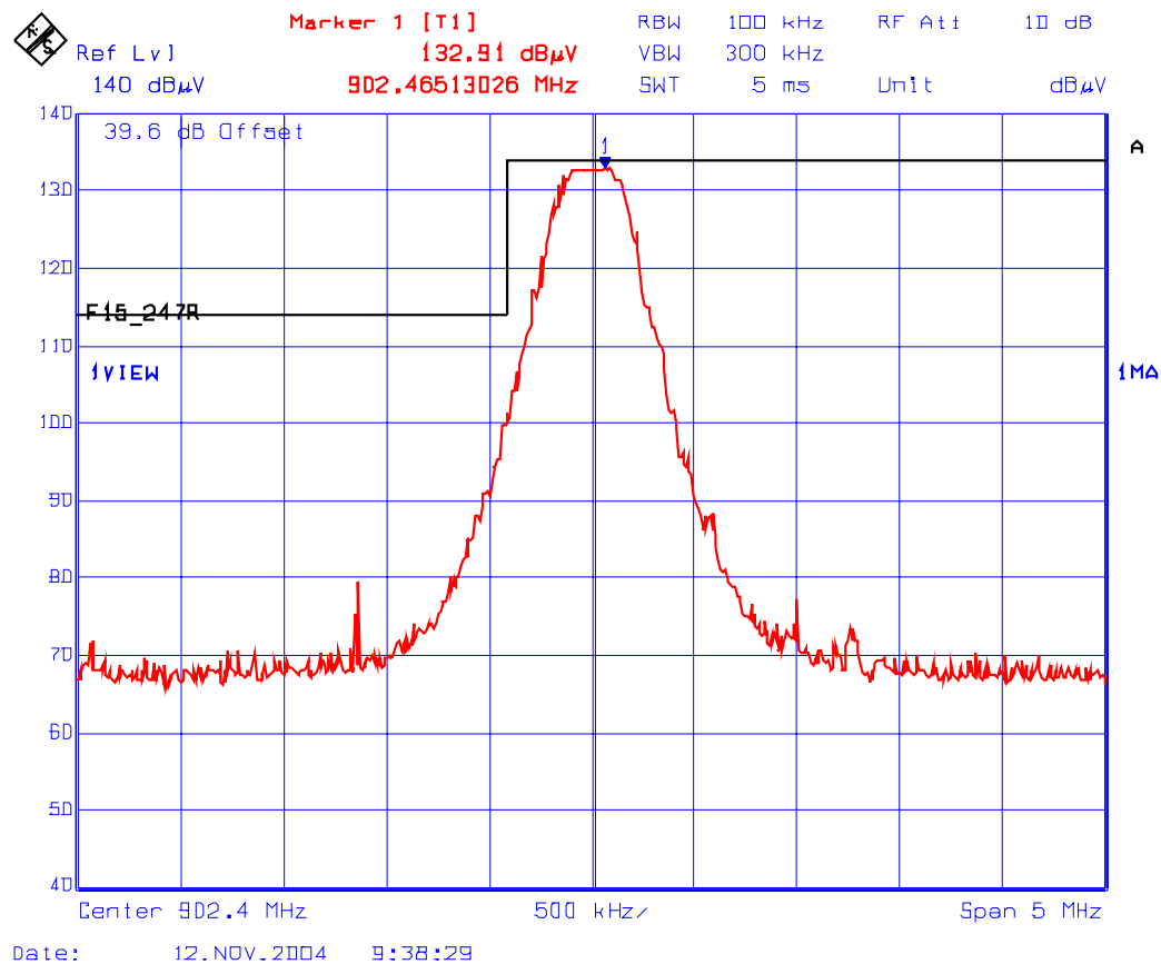
Plot 52: Band-Edge RF Radiated Emissions @ 3 meters Low End of Frequency Band Test Configuration 5: EUT with Omni Directional Antenna (8.15 dBi Gain) Rx Antenna Orientation: Vertical
