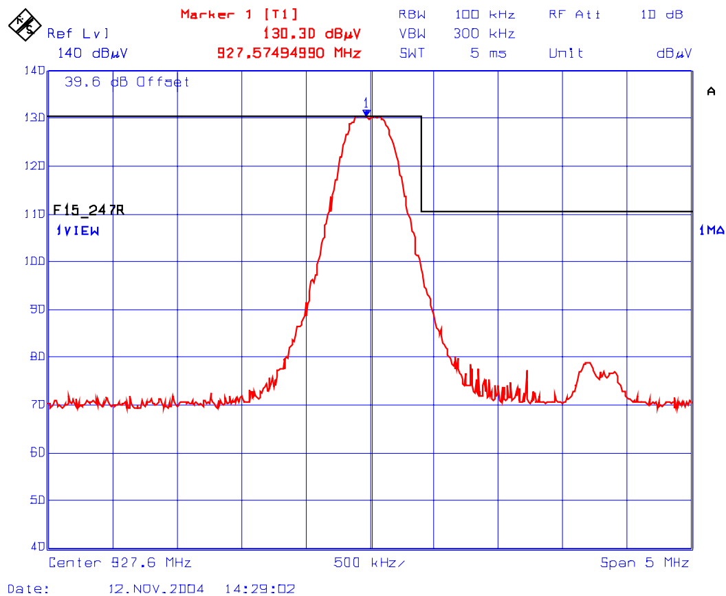
Plot 42: Band-Edge RF Radiated Emissions @ 3 meters Upper End of Frequency Band Test Configuration 2: EUT with Rubber Duck Antenna (2 dBi Gain) Rx Antenna Orientation: Vertical
