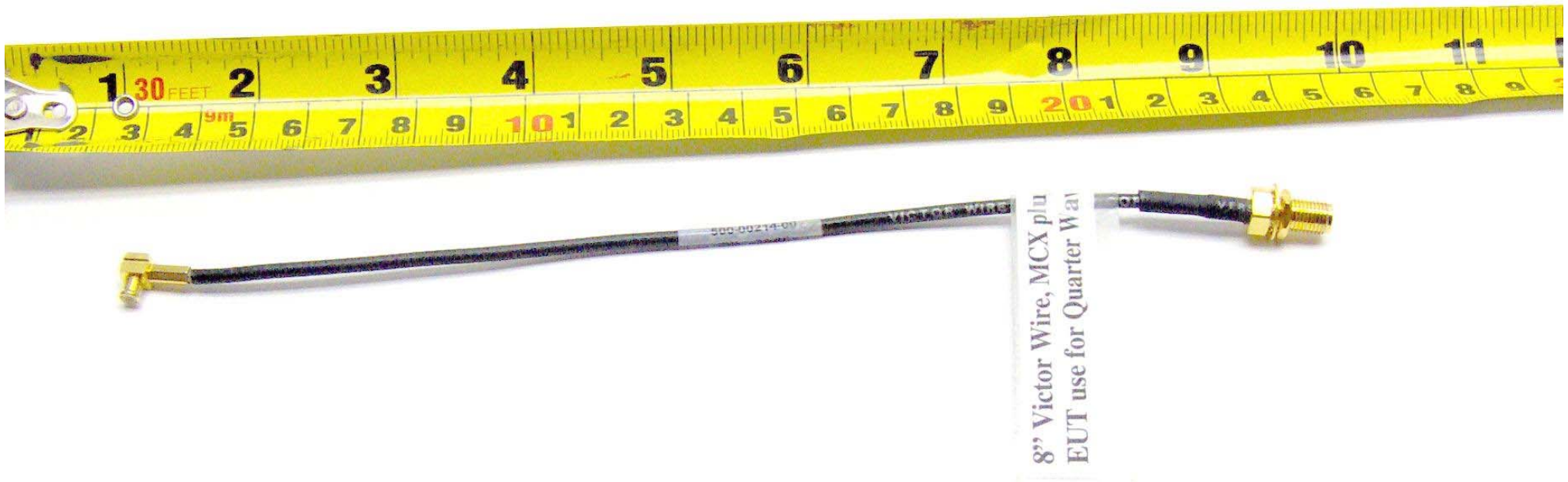
8 inch Victor Wire, MCX - RPSMA Assembly Cable
